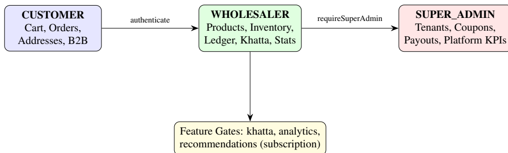
Figure 7.2: Role-Based Access Control Matrix
