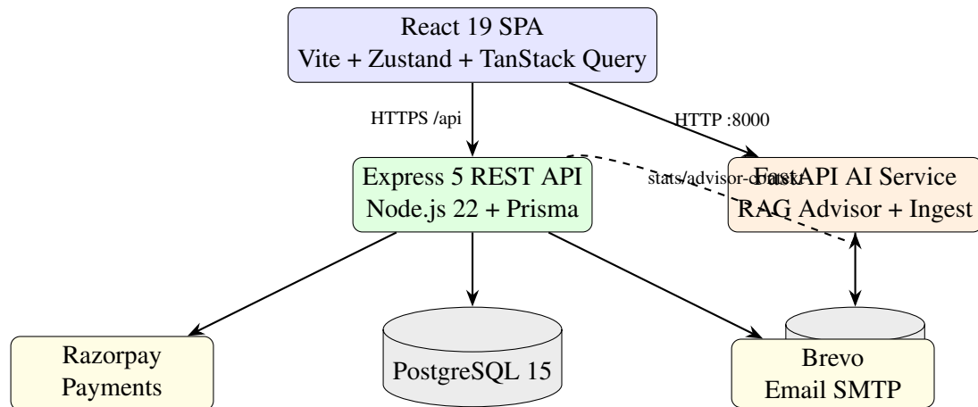
Figure 1.1: NexCart Three-Tier Architecture with AI Sidecar
