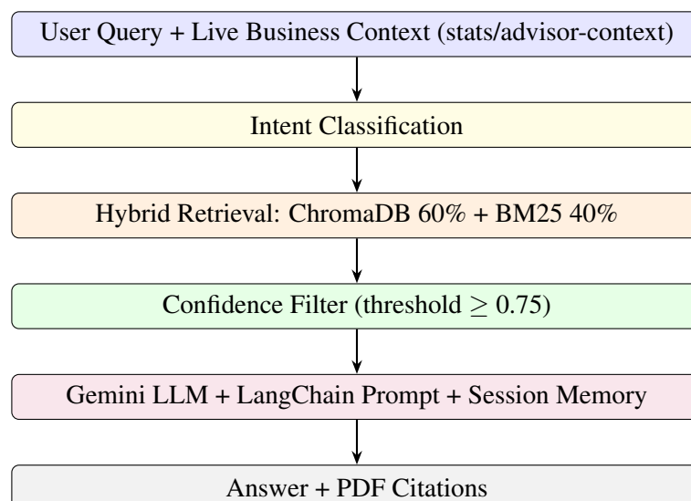
Figure 6.3: AI Business Advisor RAG Pipeline
