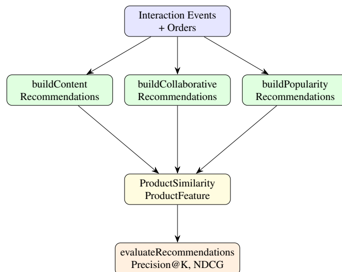
Figure 6.2: Offline Recommendation Job Pipeline
