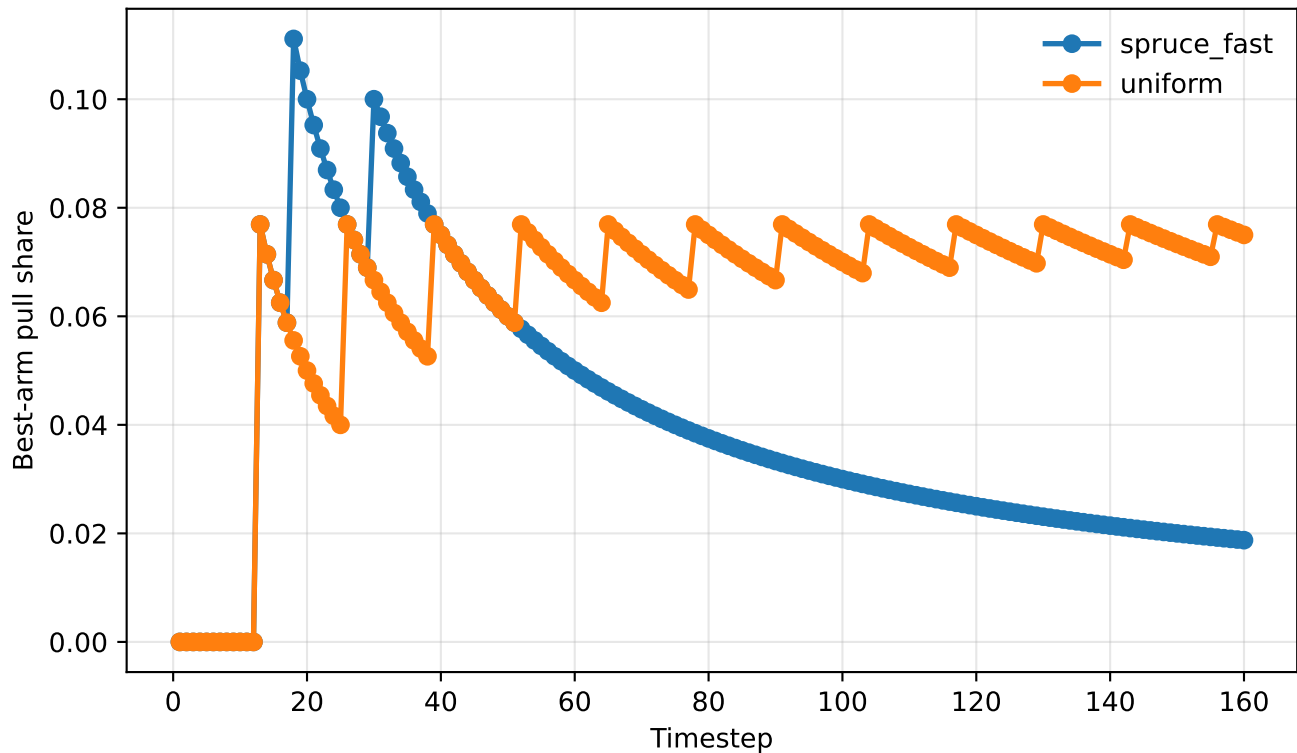
Best Arm Pull Share vs Time
