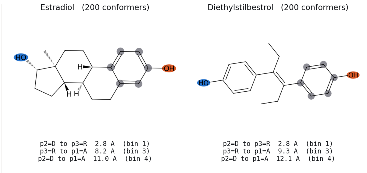
Figure 2. A mapping of one three-point pharmacophore onto (i) estradiol (top), the natural ligand, and (ii) diethylstilbestrol (bottom). The hydroxyl groups are both hydrogen bond donors and acceptors (D, A), and the centroid of the aromatic ring is shown (R). The two molecules share no scaffold, yet present the same three features at distances that fall in the same bins, so the same bit is set in both. Reproduced from reference 1.
