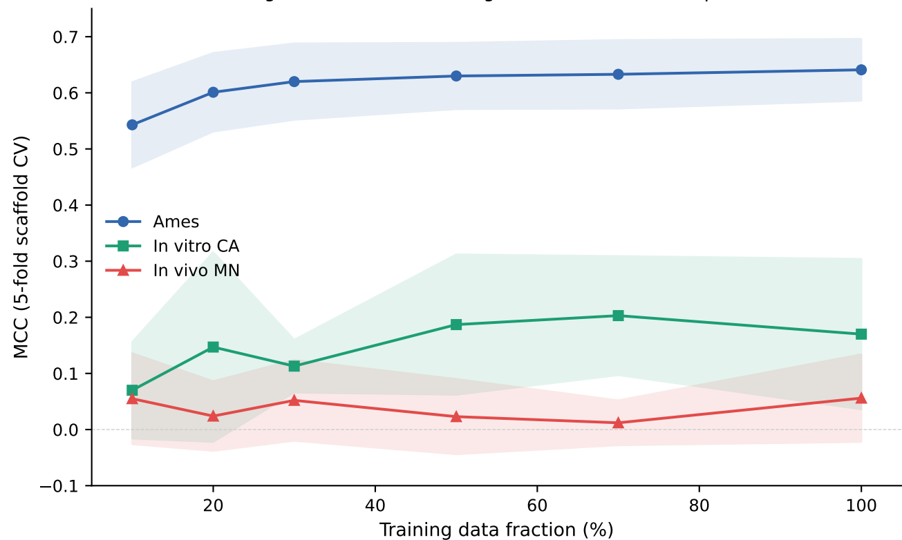
Learning curves — locked configuration (XGBoost, compact, raw)
