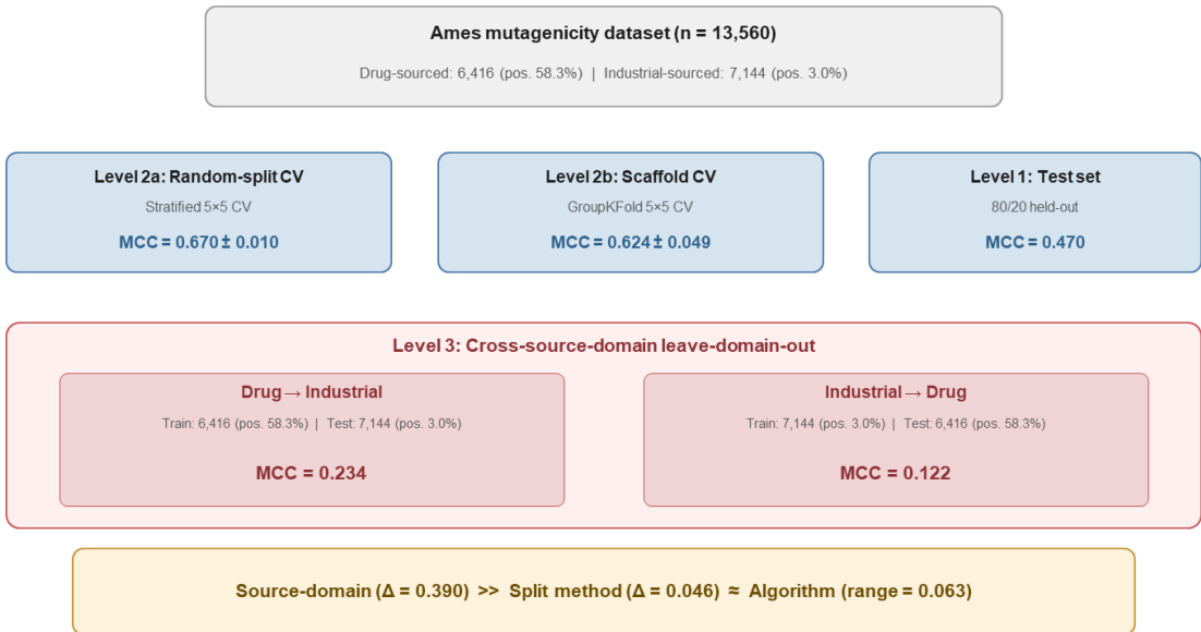
Figure 1: Evaluation cascade framework. All levels use the same fixed configuration (XGB, compact features, raw SMILES), enabling fair MCC comparison across evaluation methods.
