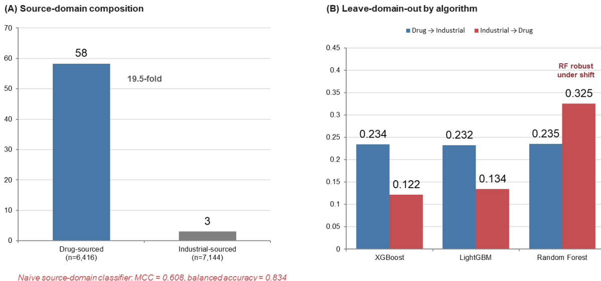
Figure 4: Data source heterogeneity in Ames. (A) Positive rate by source: drug 58.3% vs. industrial 3.0% (19.5-fold). (B) LDO MCC by algorithm; Random Forest is substantially more robust in the industrial→drug direction.
