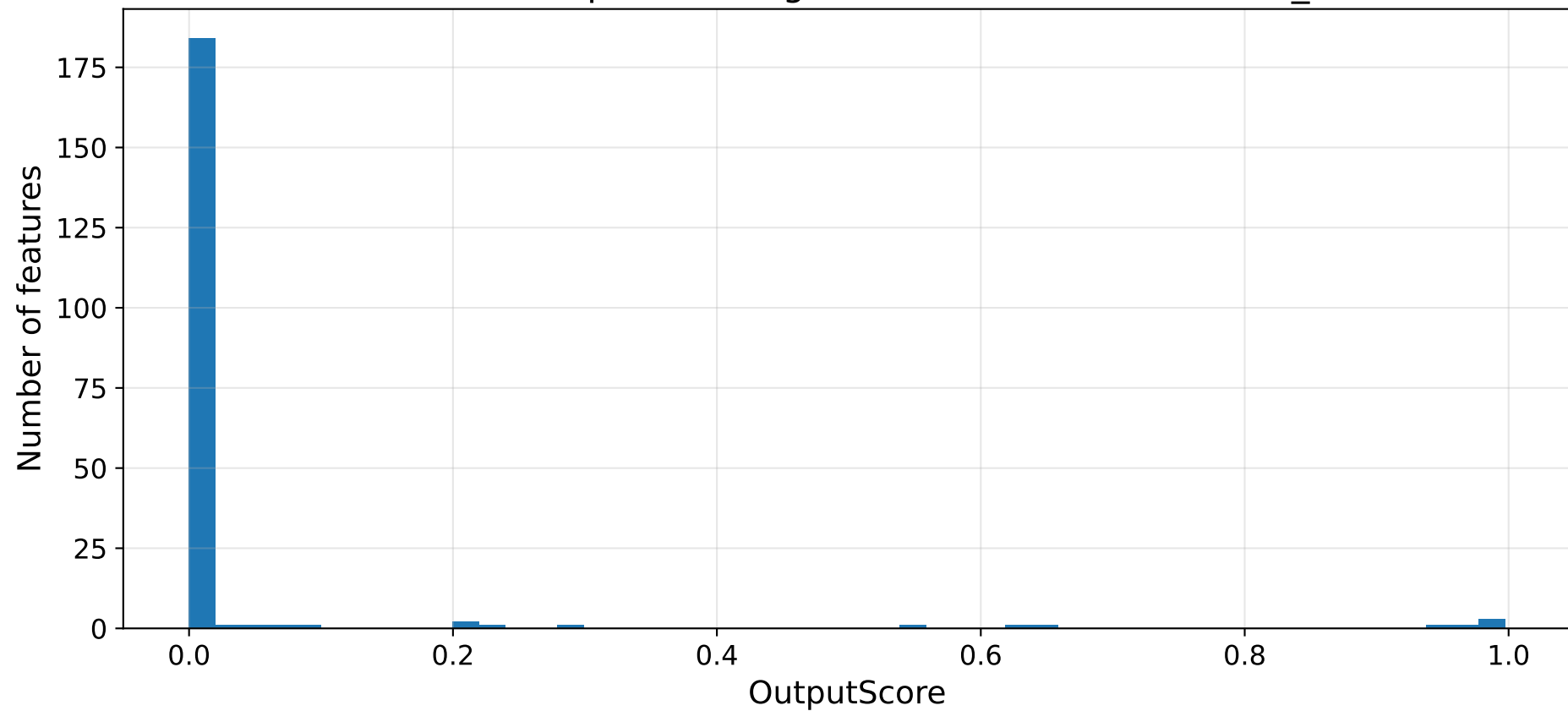
Distribution of OutputScore · gemma-2-9b-it · vocab=clar_vocab2
