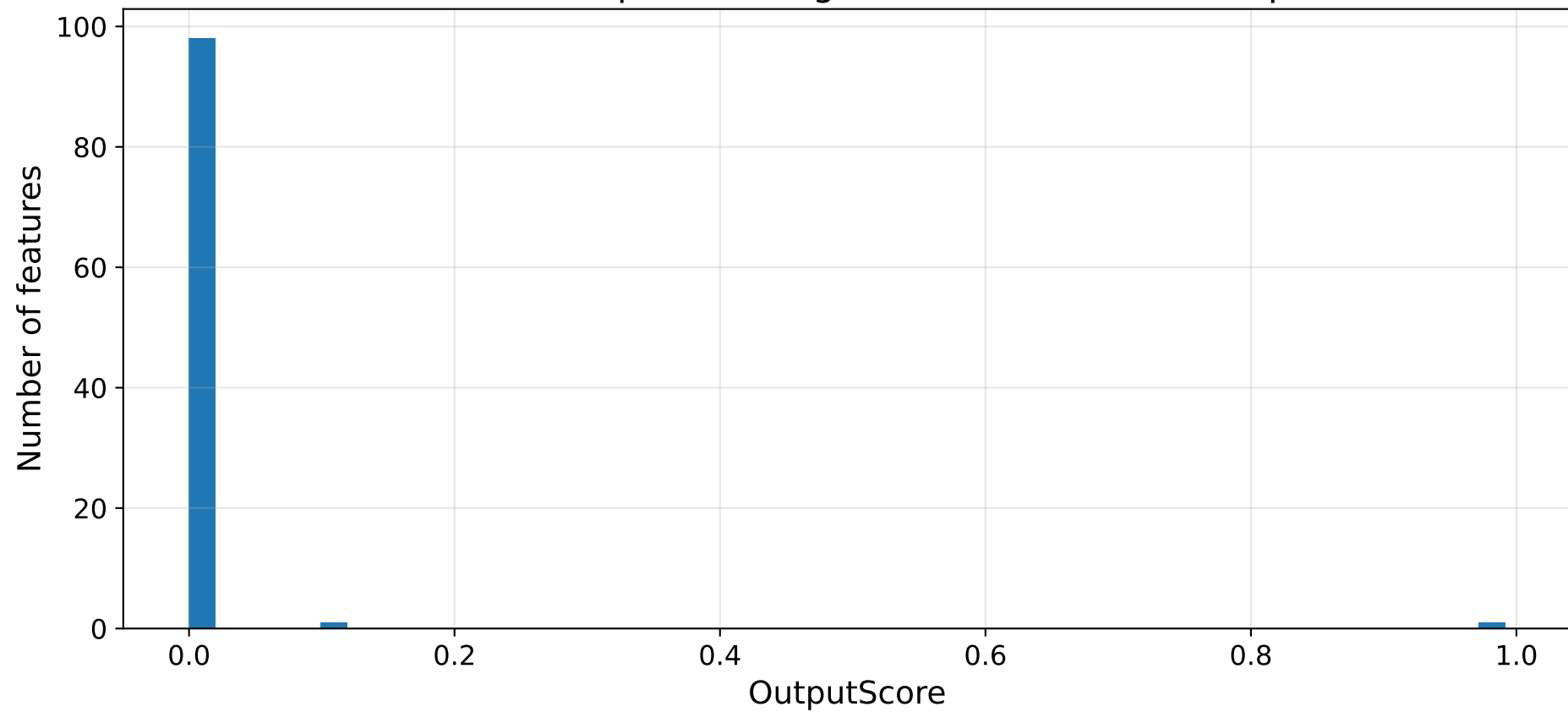
Distribution of OutputScore · gemma-2-9b-it · vocab=question
