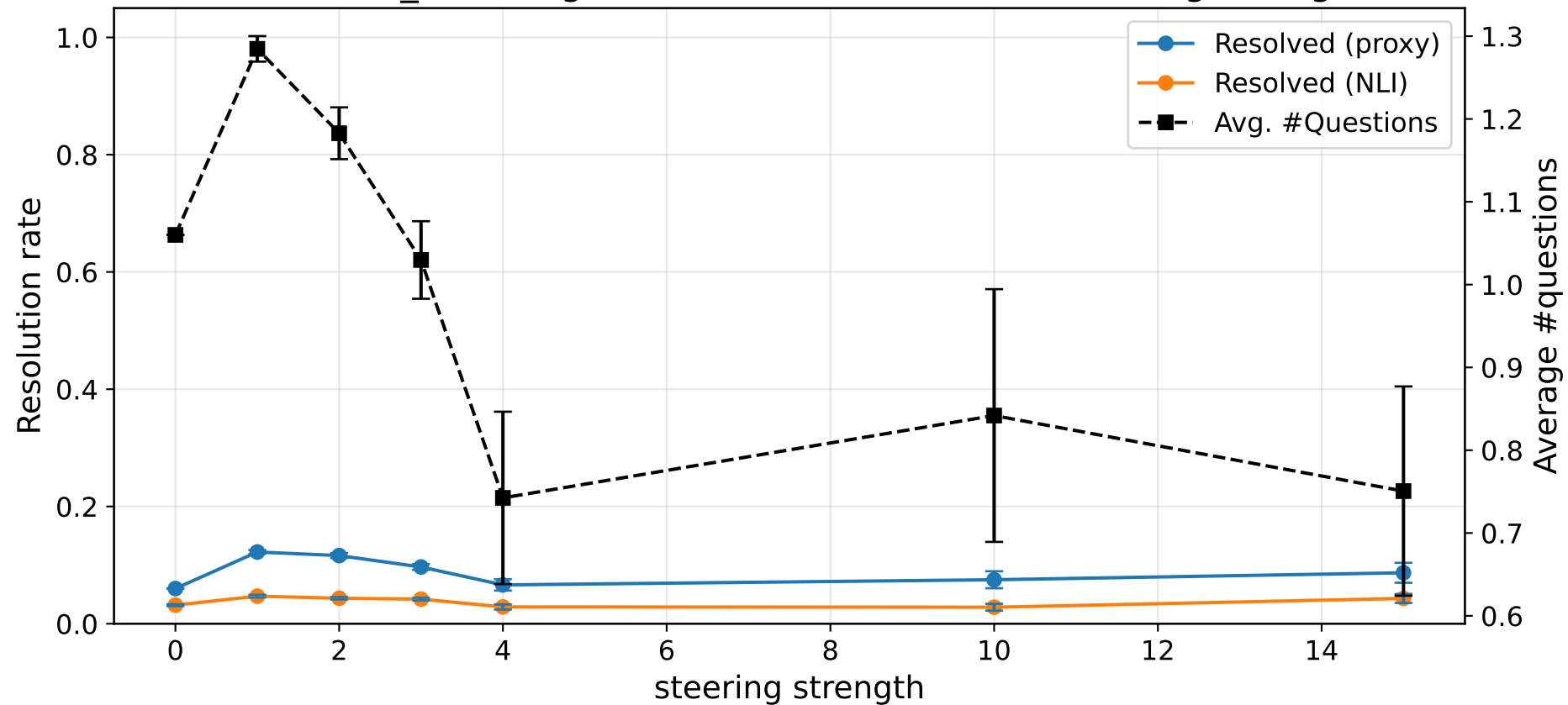
AmbiK-clar_vocab · gemma-2-9b-it · metrics vs steering strength
