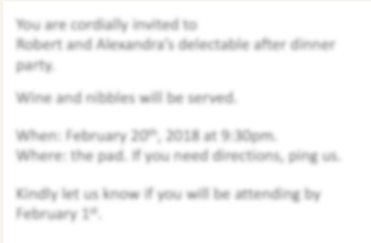
Conceptual grouping
