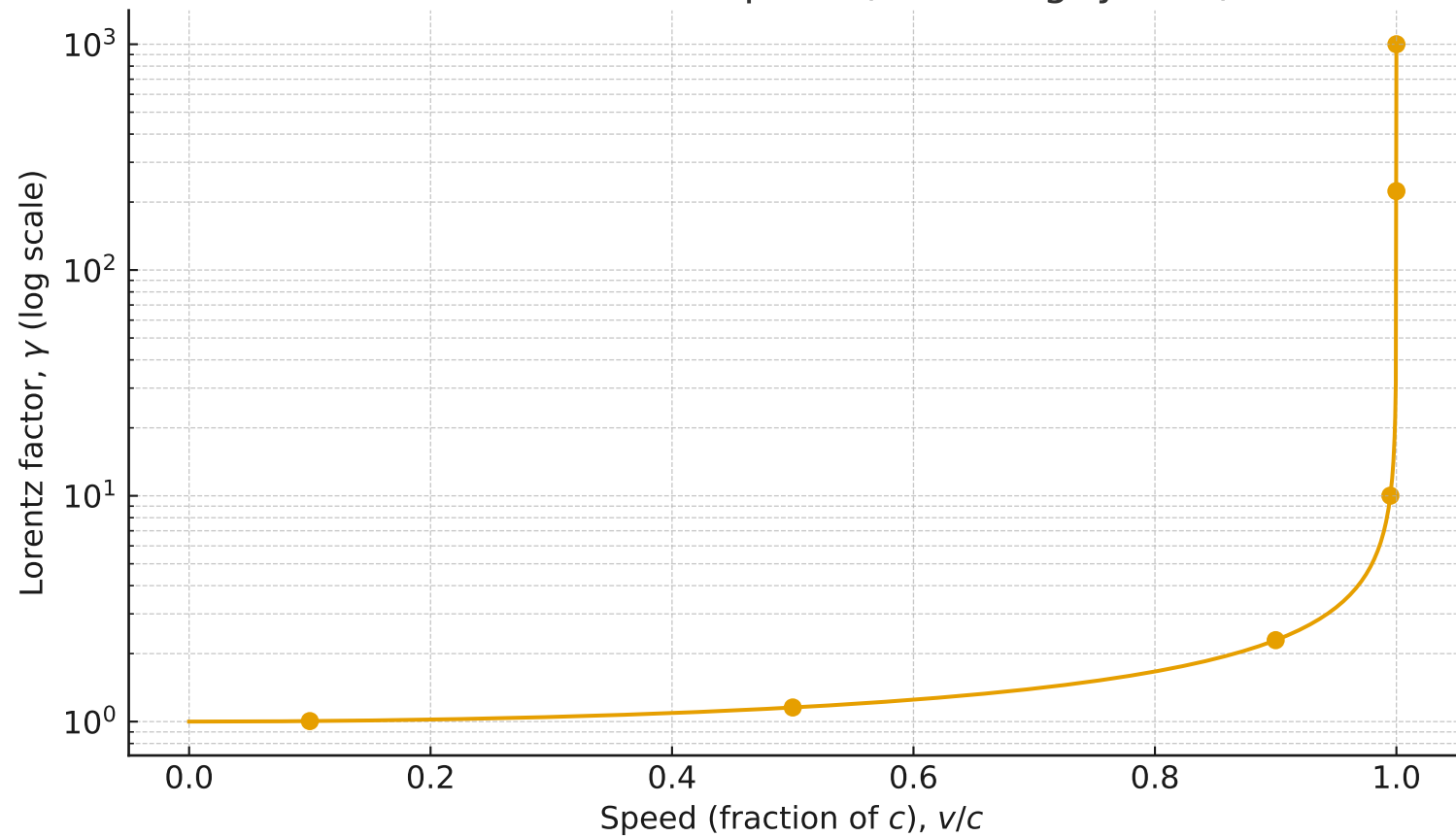
Lorentz Factor vs Speed (Semi-Log: y-axis)
