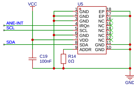
Differential Pressure Sensor
