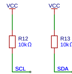
I2C Pull-up
