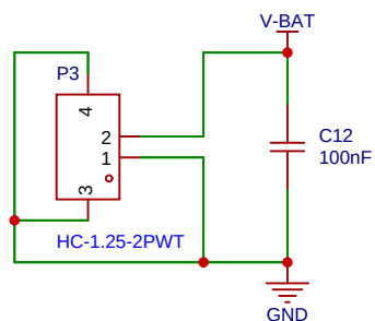
Li-ion Battery Connector
