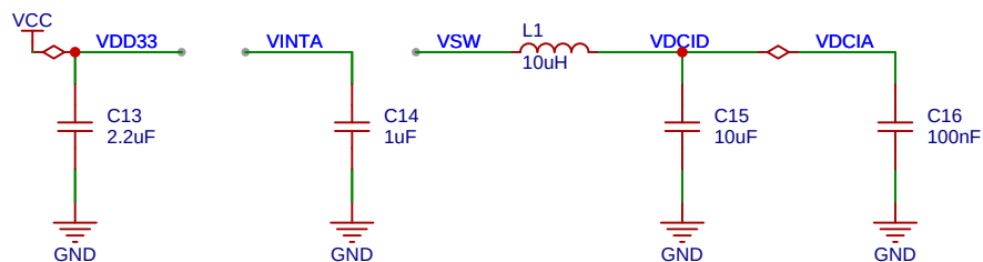
Power & On-chip DC-DC
