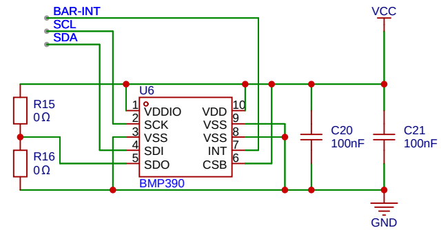
Air Pressure Sensor
