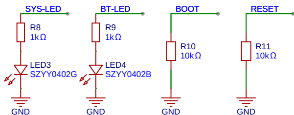
LEDs & System Pins
