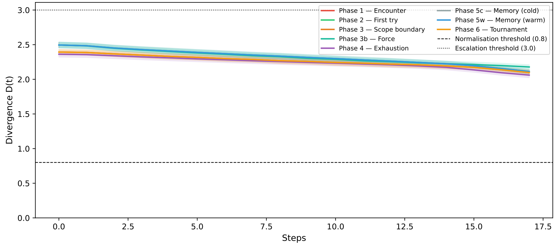
PERSIST: Divergence signal across experimental phases (n=5 seeds, mean \pm std)
