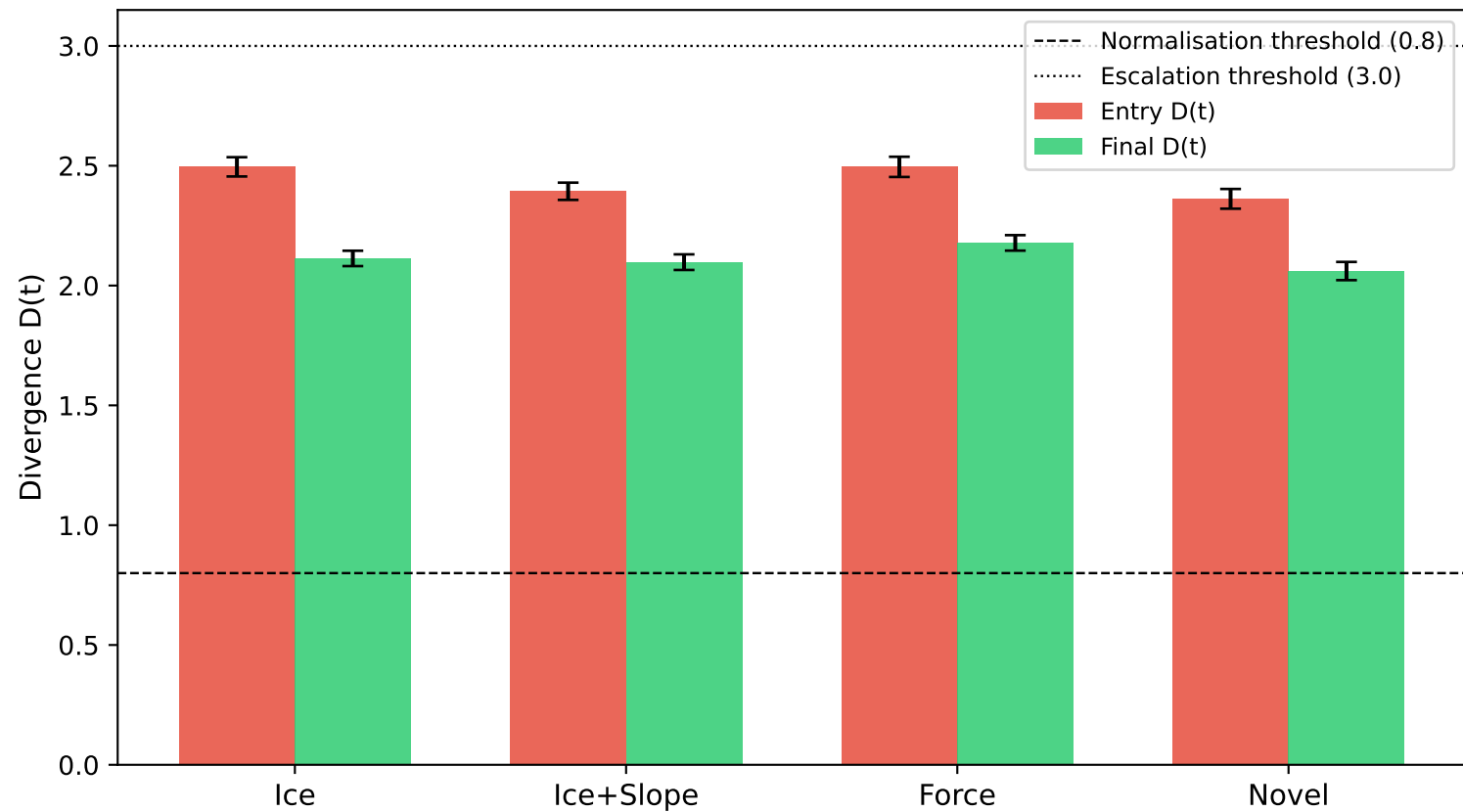
Zone detection: entry vs resolved D(t) (n=5 seeds, mean \pm std)
