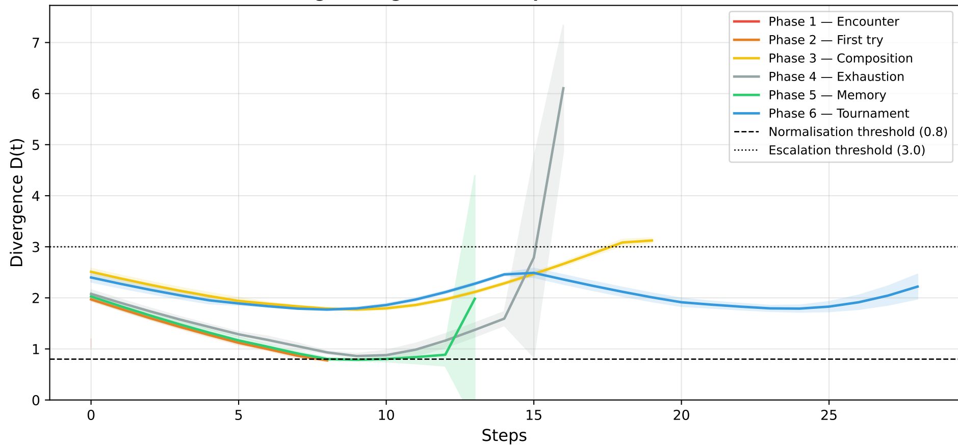
PERSIST: Divergence signal across six phases (n=5 seeds, mean \pm std)
