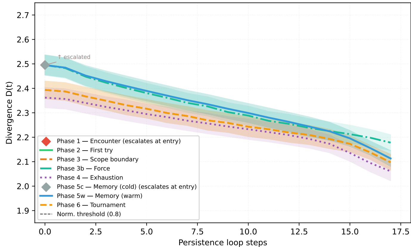
D(t) across experimental phases (n=5 seeds, mean \pm std)
