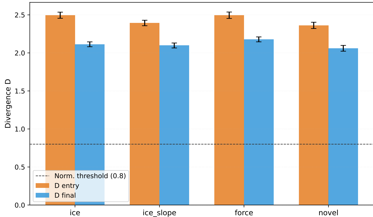
Zone detection: entry vs final D (n=5 seeds, mean \pm std)
