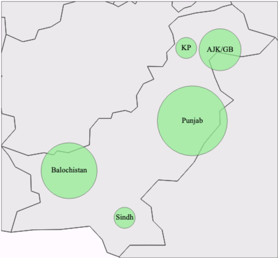
Bubble Map for Responses
