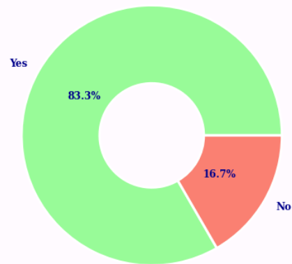
Satisfied with Resolution?
