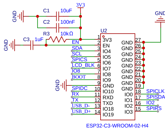
ESP32-C3-WROOM-02-H4
