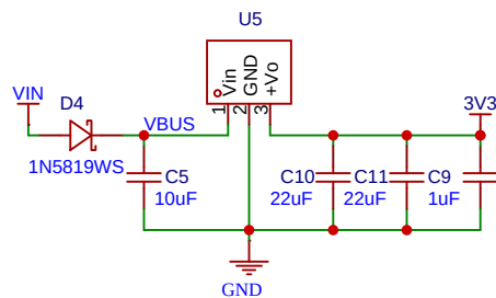
Power DC-DC 24-3.3V
