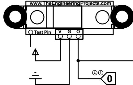
SENSOR PROXIMITY CAPACITIVE
