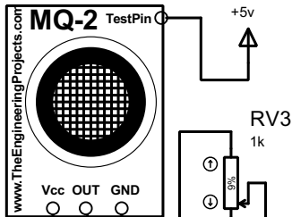
MQ2 GAS SENSOR
