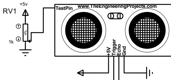
SONAR1 ULTRASONIC SENSOR
