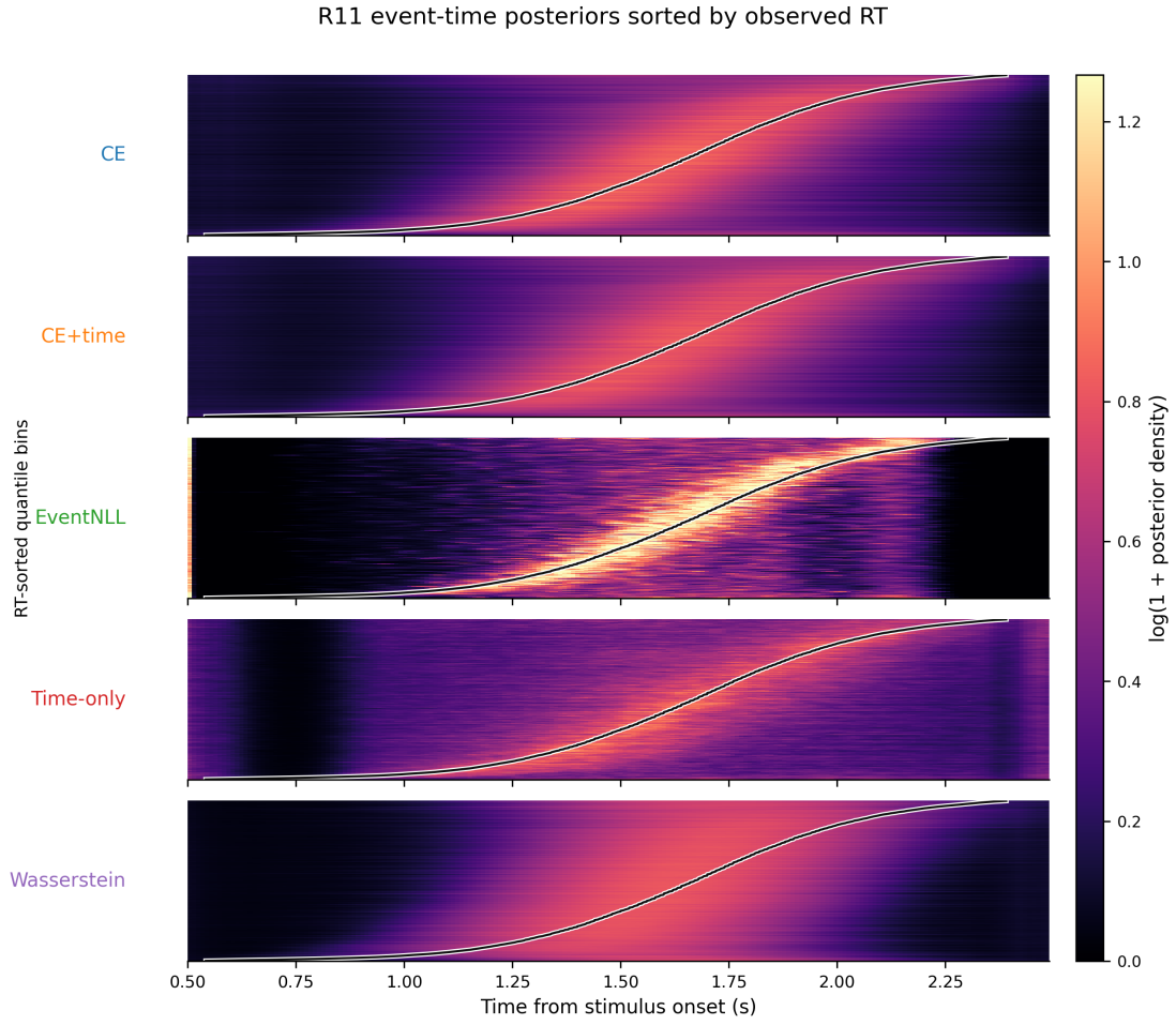
Figure 9: Trial-sorted event-time posterior maps on R11 for matched segmentation losses. Rows are quantile bins of representable R11 trials sorted by observed RT; the x-axis is time from stimulus onset; color shows log-transformed posterior density averaged within each bin. The black curve marks the mean observed RT in each bin.
