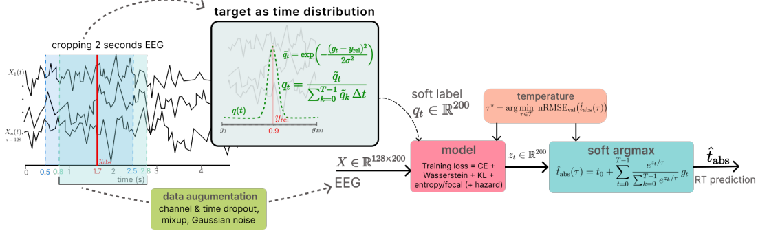
Figure 4: Temporal segmentation pipeline for RT prediction. For each trial we cache a longer stimulus-locked segment (4 s in our implementation) and sample a 2 s subwindow with start-time jitter for training; the RT label is shifted into the sampled window and a Gaussian soft target q_t is formed. Per-time logits z_t are produced by a 1-D segmentation model and are optimized with distribution-matching losses (e.g., soft-label CE, CDF-based Wasserstein-1, KL, and mild entropy penalty) or latent EventNLL objectives. The main readout is a temperature-scaled softmax posterior; hazard/survival readouts and alternate observation kernels are evaluated as compact extensions. RT is obtained by temperature-scaled soft-argmax, with \tau^* selected to minimize validation nRMSE.
