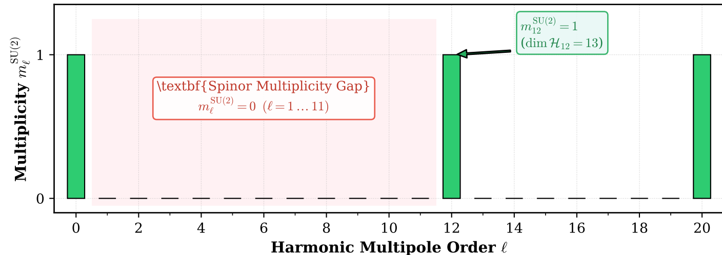
(b) Full Spinor Spectral Eigenmodes on S^3/I^* [SU(2) Character Projector]
