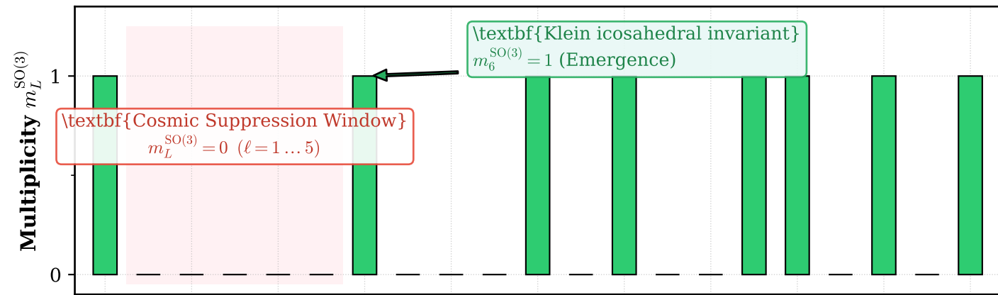
(a) Physical Spherical Harmonics on SO(3) / CMB Multipole Modes
