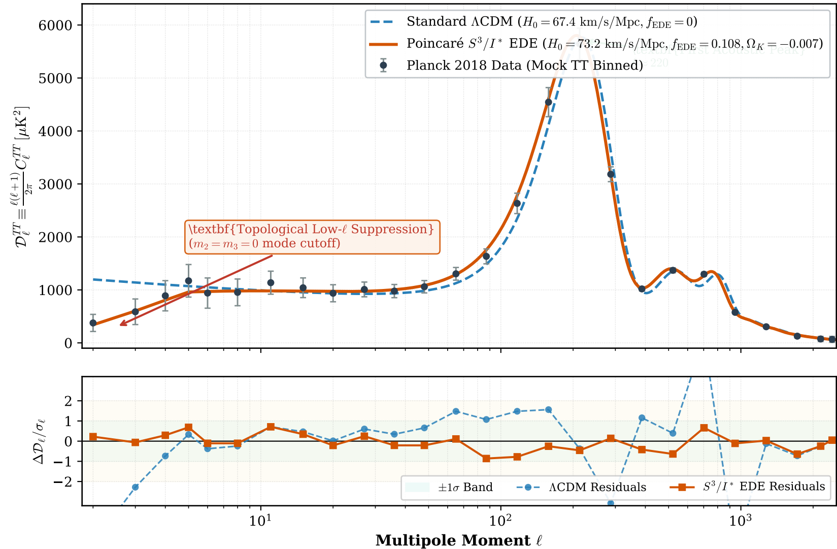
\textbf{CMB Temperature Power Spectrum C_\ell^{TT} : Poincaré S^3/I^* EDE vs. Standard \Lambda CDM}
