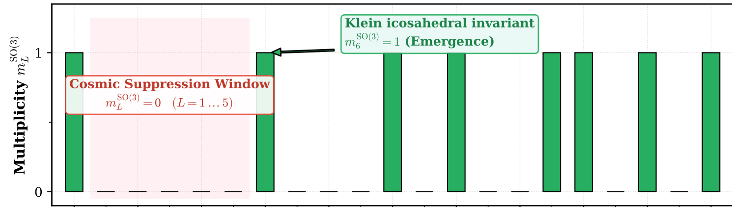
(a) Physical Spherical Harmonics on SO(3) / CMB Multipole Modes
