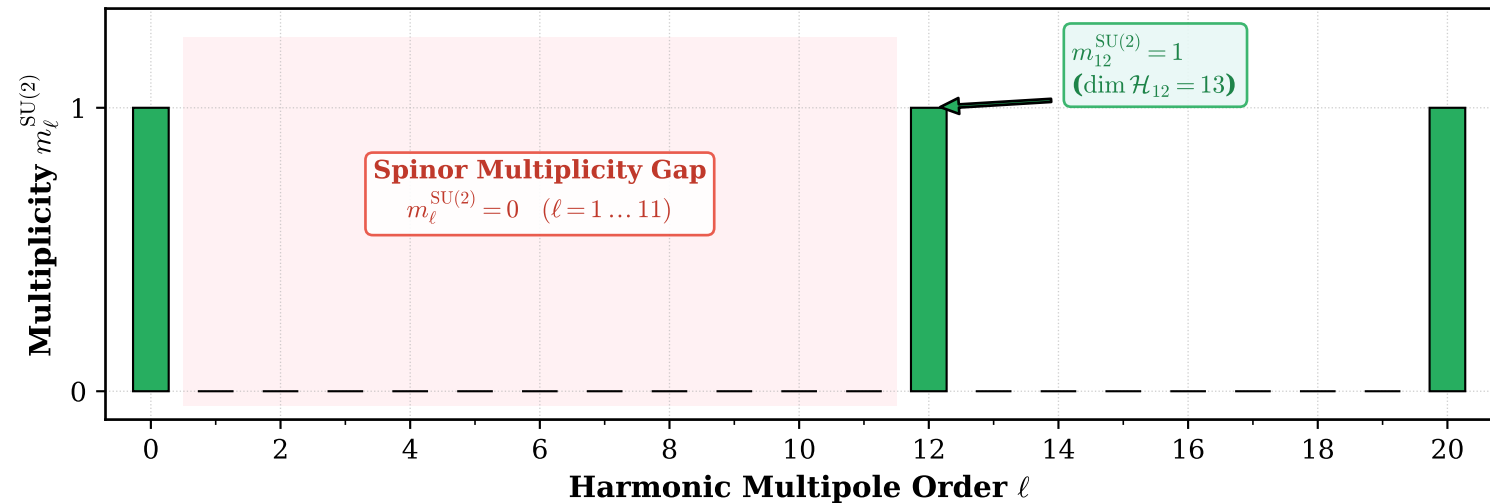
(b) Full Spinor Spectral Eigenmodes on S^3/I^* [SU(2) Character Projector]
