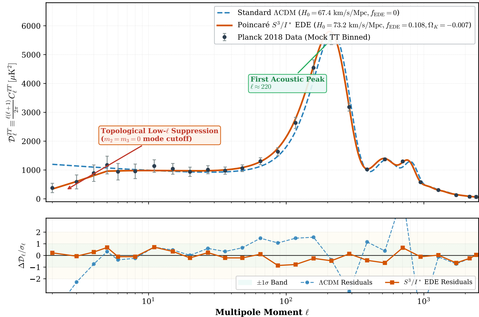
CMB Temperature Power Spectrum \mathcal{D}_\ell^{TT} : Poincaré S^3/I^* EDE vs. Standard \Lambda CDM
