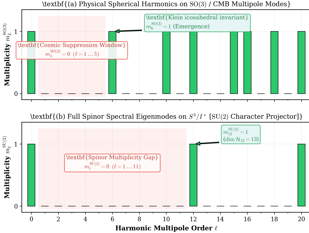
Figure 1: Exact multipole invariant multiplicities on \frac{S^3}{I^*} computed via Molien's character projection formula. Panel (a) shows physical SO(3) spherical harmonics with exact vanishing for L = 1 \dots 5 and emergence at L = 6 . Panel (b) shows the full SU(2) spinor spectrum exhibiting the 11-mode gap with first emergence at \ell = 12 .
