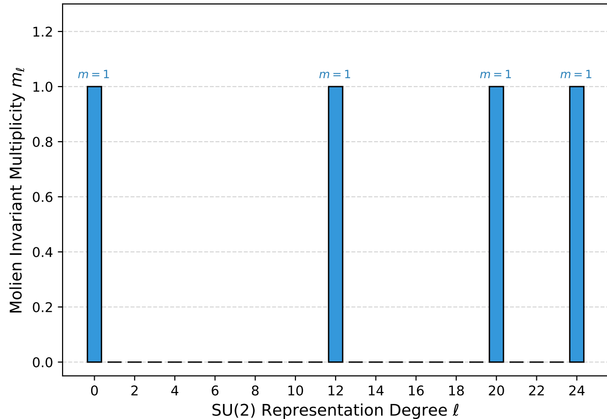
(b) Full Spinor Harmonics on S^3/I^* (Molien Invariants)
