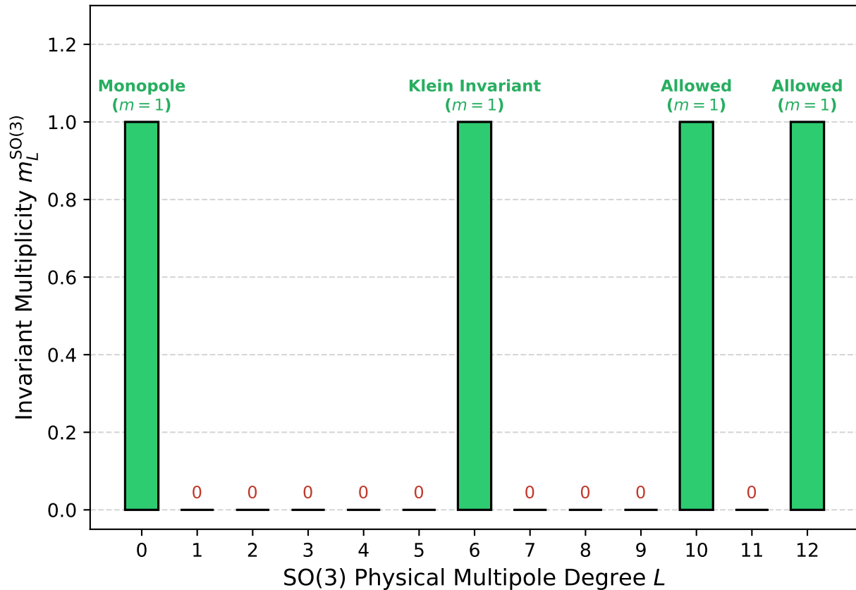
(a) Physical CMB Harmonics on \mathcal{M}^3 = S^3/I^*
