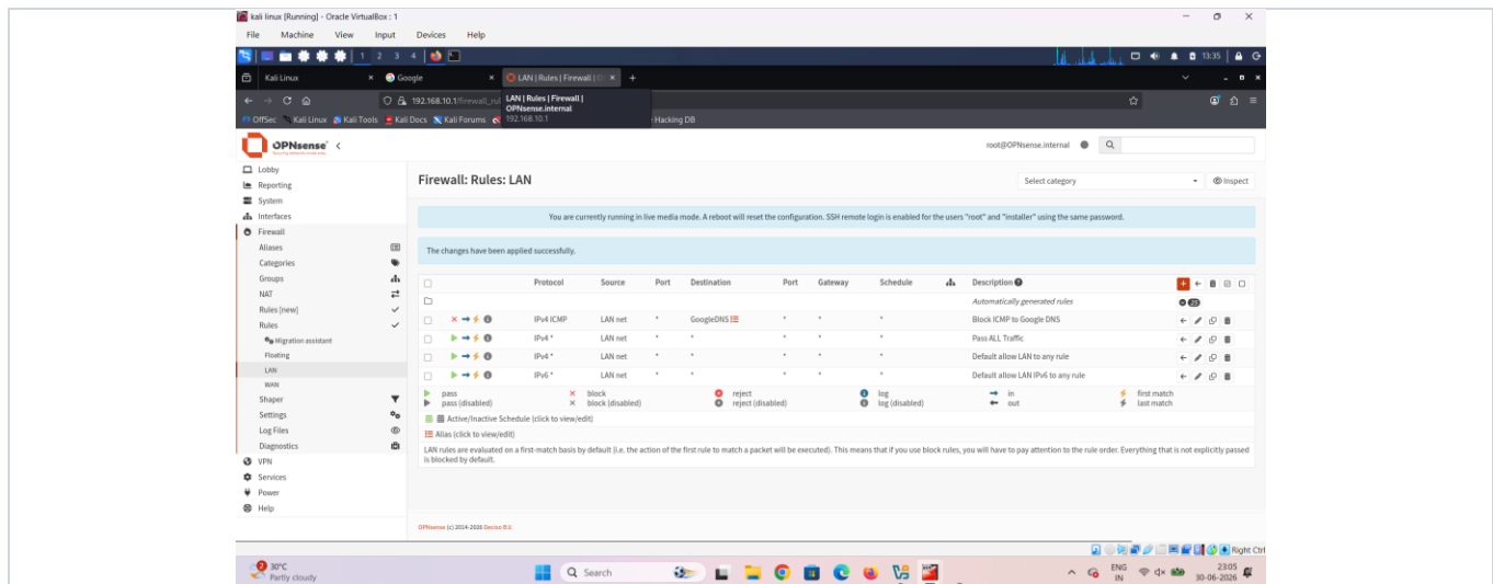
Figure 6: Firewall › Rules › LAN after correcting the order: “Block ICMP to Google DNS” is once again evaluated before “Pass ALL Traffic” and the default allow rules, restoring the intended block behaviour.
