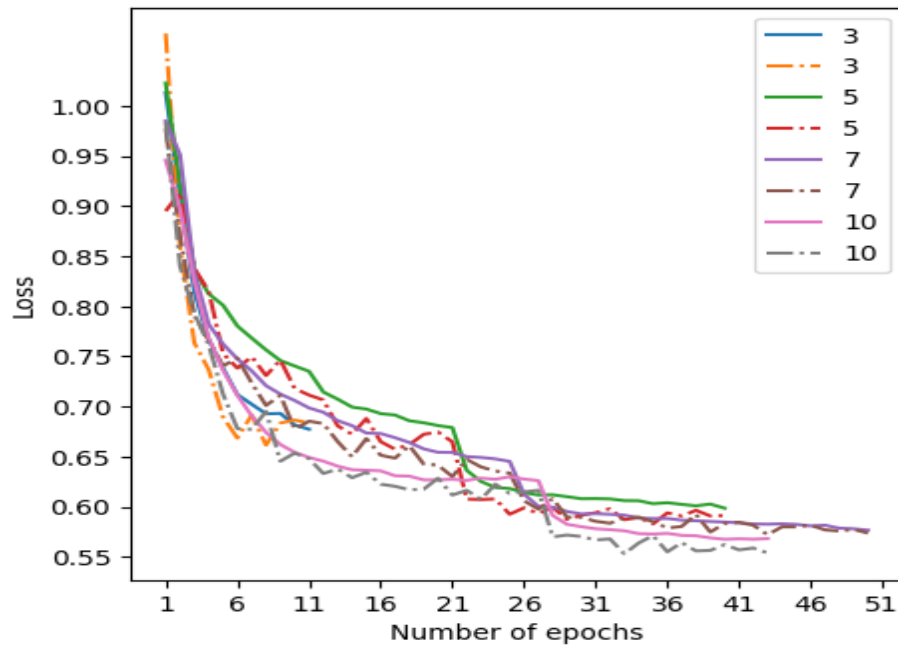
Figure 5.2.4: Overview of the validation loss of the models trained with different values of the patience parameter in early stopping when dimension of the latent space representation was fixed to 512, the number of semantic subgroups is 32 and batch size is 128. The y-axis represents the loss. The x-axis represents the number of number of epochs. The solid lines represent the mean training loss after each epoch. The dash dot line represents the mean validation loss after each epoch. The numbers in the legend represent the value of the patience parameter.
