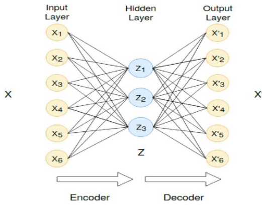
Figure 3.2.2: Architecture of an undercomplete autoencoder.[51]
