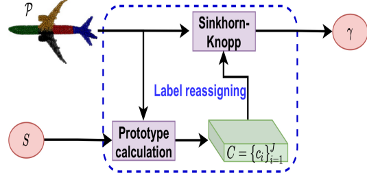
Figure 4.1.9: Architecture of label reassigning [55]
