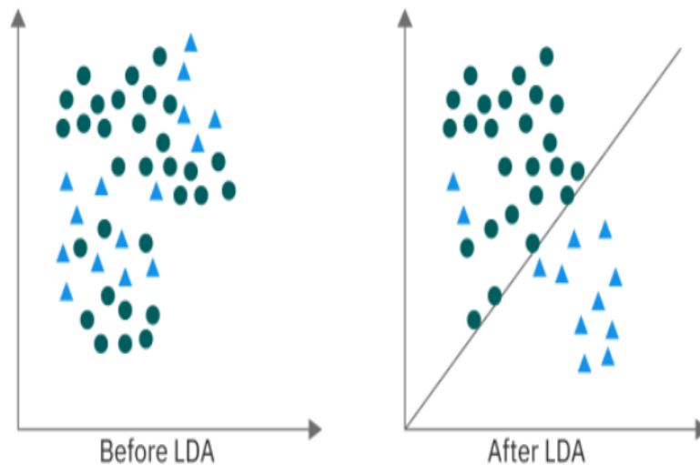
Figure 3.6.2: Projection of the data before and after applying LDA.[102]
