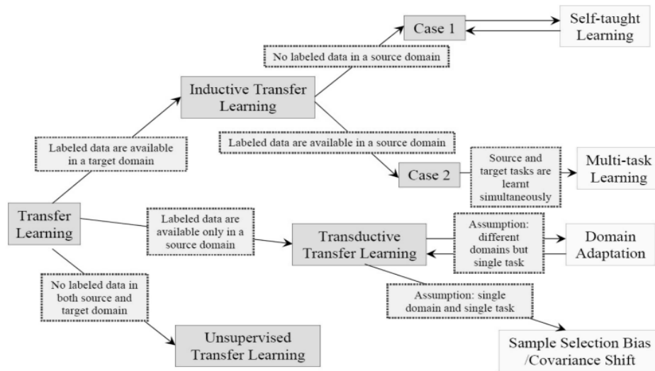
Figure 3.5.3: Overview of the different types of transfer learning.[54]
