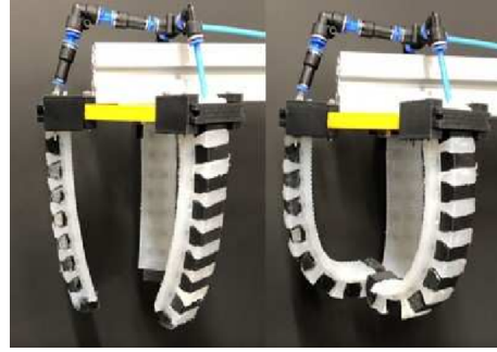
Figure 3.1.6: Hybrid Grippers with soft and rigid structures[56]
