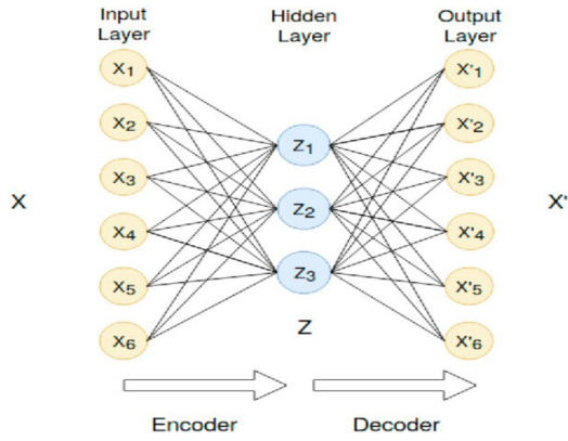
Figure 3.2.1: Architecture of an undercomplete autoencoder.[48]
