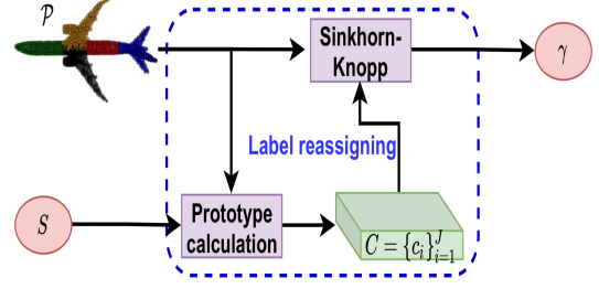
Figure 4.3.3: Architecture of label reassigning [47]
