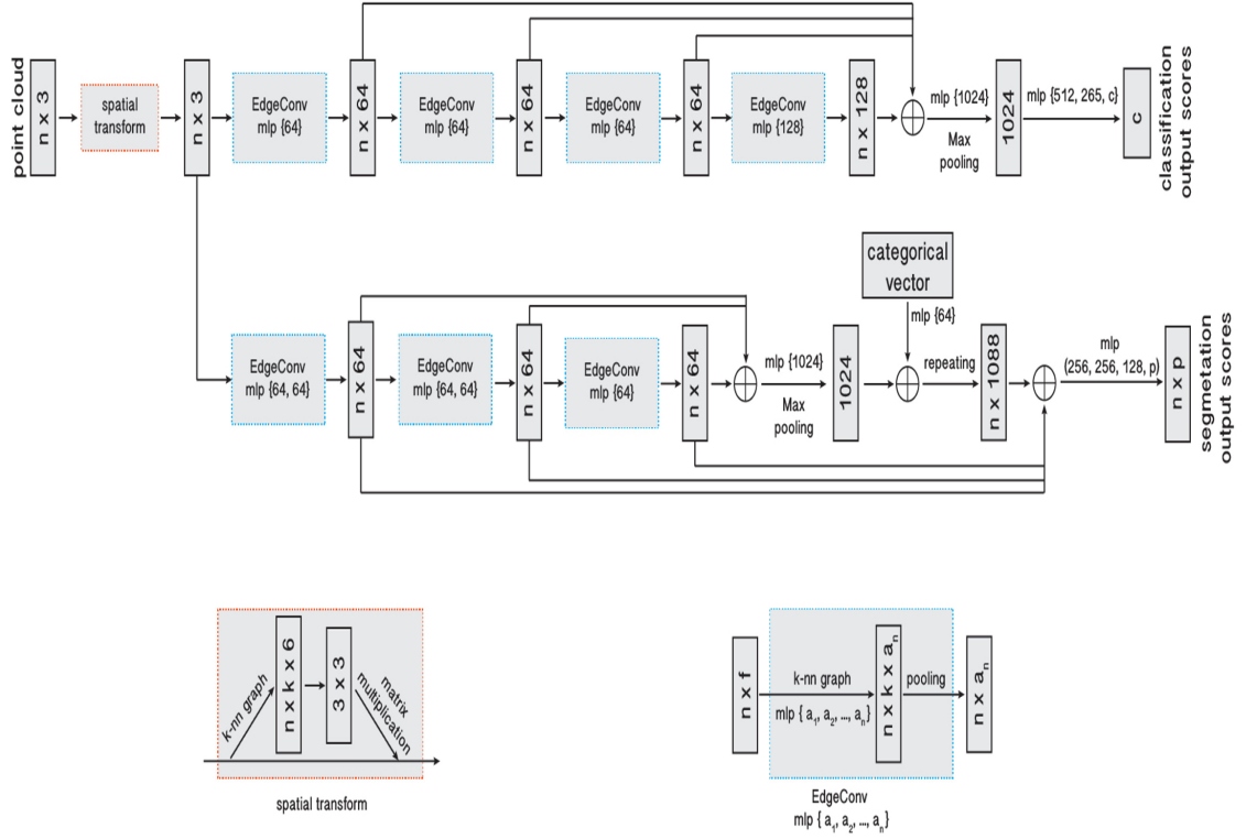
Figure 4.2.3: The DGCNN Architecture.[77]
