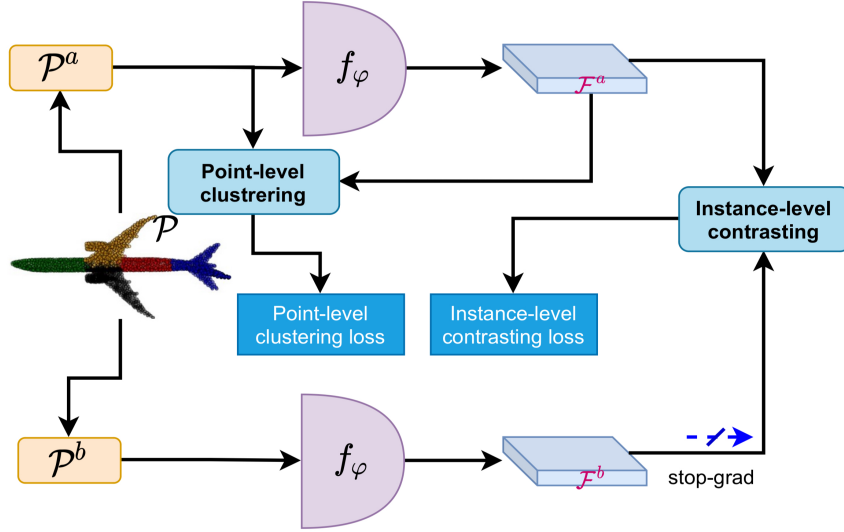
Figure 4.1.1: The Conclu model pipeline including the two modules: point -level clustering and instance-level contrasting.[47]
