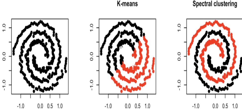
Figure 3.3.4: A comparison between the results of K-means clustering and Spectral clustering. The image in the left shows the points that need to be clustered. [53]
