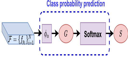
Figure 4.3.2: Architecture of class probability prediction.[47]
