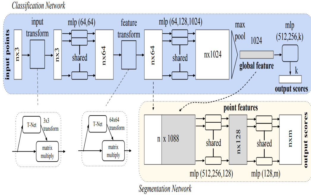
Figure 4.2.1: The PointNet Architecture.[60]
