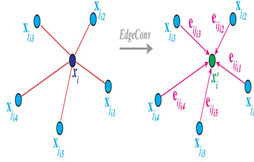
Figure 4.2.5: The EdgeConv operation. The output of EdgeConv is computed by aggregating the features associated with all the edges that originate from each connected vertex. [77]
