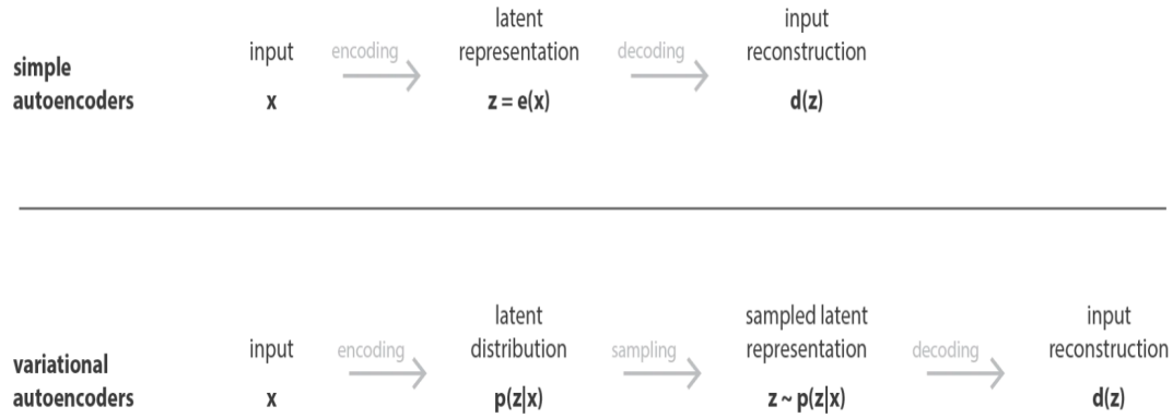
Figure 3.2.3: Difference between a vanilla autoencoder and a Variational Autoencoders (VAE).[72]
