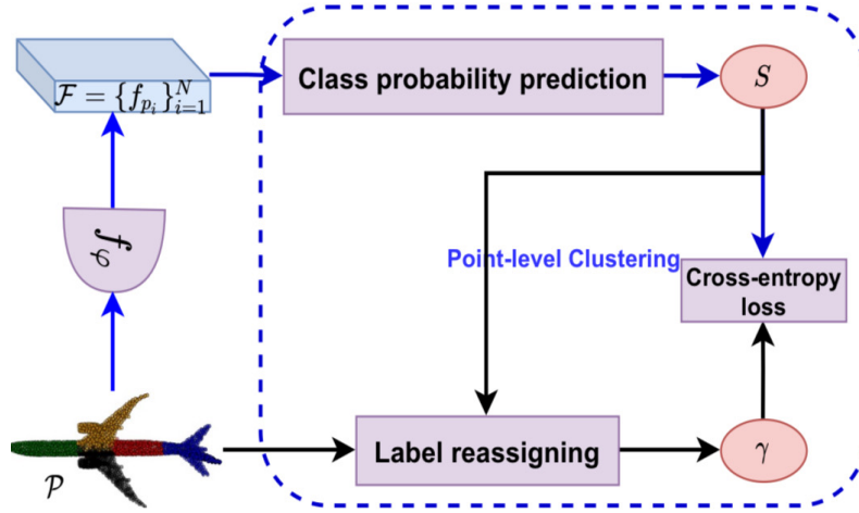
Figure 4.3.1: The architecture of the point-level clustering based unsupervised feature learning.[47]
