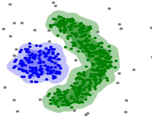
Figure 3.3.1: DBSCAN can find non-linearly separable non-convex clusters.[15]
