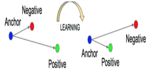
Figure 3.2.5: Before (left) and after (right) minimizing triplet loss function[71]
