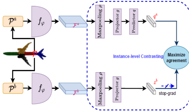
Figure 4.4.1: The architecture of the instance-level Contrasting.[47]
