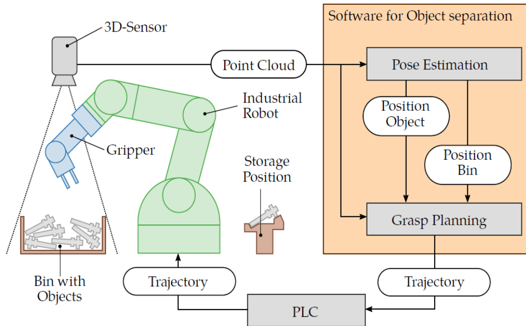
Figure 3.1.7: Overview of model-based bin picking approach.[68]
