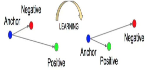
Figure 3.2.6: Before (left) and after (right) minimizing triplet loss function[78]
