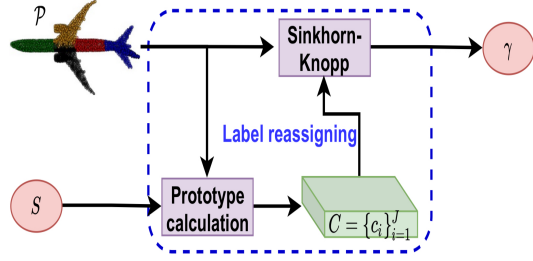
Figure 4.1.9: Architecture of label reassigning [55]
