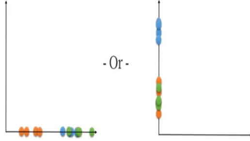
Figure 4.2.2: Data projected to 1-D space [90].
