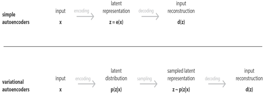
Figure 3.2.4: Difference between a vanilla autoencoder and a Variational Autoencoders (VAE).[93]
