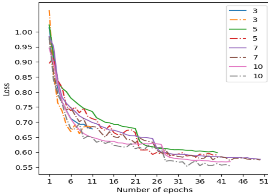
Figure 5.2.4: Overview of the validation loss of the models trained with different values of the patience parameter in early stopping when dimension of the latent space representation is fixed to 512, the number of semantic subgroups is 32 and batch size is 128. The y-axis represents the loss. The x-axis represents the number of epochs. The solid lines represent the mean training loss after each epoch. The dash dot line represents the mean validation loss after each epoch. The numbers in the legend represent the value of the patience parameter.
