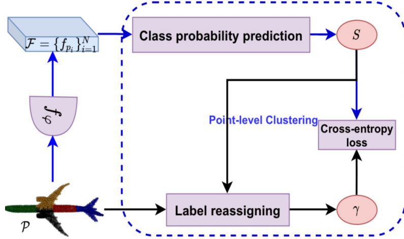
Figure 4.1.7: The architecture of the point-level clustering based unsupervised feature learning.[55]
