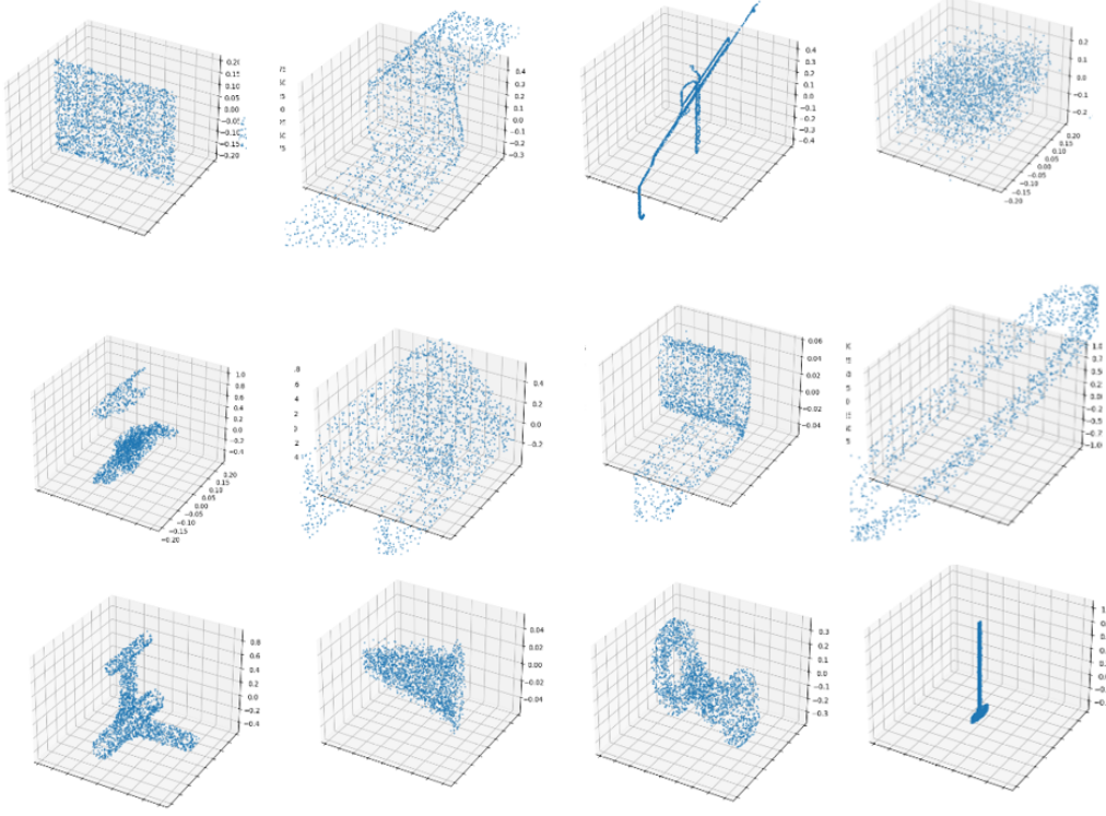
Figure 5.5.1: Some of the representative members of the ABC dataset[44] obtained on applying multi-level HDBSCAN algorithm on the feature representations obtained from the ConClu approach with PointNet Autoencoder backbone.
