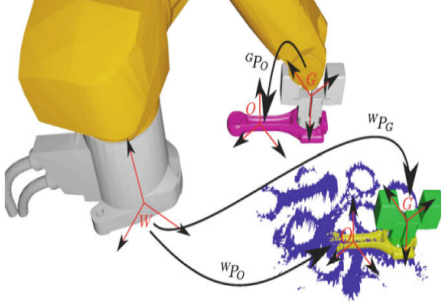
Figure 3.1.8: Important positions the workspace in a bin-picking application. W is the world coordinate system with it's origin at the centre of the base of the robot. O is the object coordinate system with it's origin at the center of the object. G is the gripper coordinate system with its origin at the center of the gripper. \mathbf{W}_{P_O} is the object's position in relation to the world coordinate system. \mathbf{W}_{P_G} is the end-effector's position in relation to the world coordinate system. \mathbf{G}_{P_O} is the position of the object in relation to the position of the gripper.[8]
