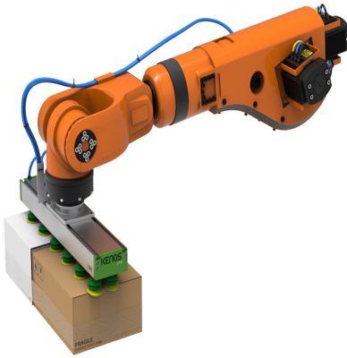
Figure 3.1.1: Vacuum Grippers[59]
