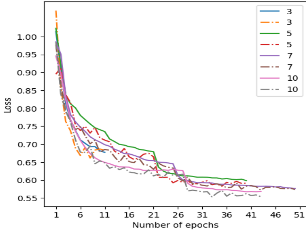
Figure 6.2.4: Overview of the validation loss of the models trained with different values of the patience parameter in early stopping when dimension of the latent space representation was fixed to 512, the number of semantix subgroups is 32 and batch size is 128. The y-axis represents the loss. The x-axis represents the number of number of epochs. The solid lines represent the mean training loss after each epoch. The dash dot line represents the mean validation loss after each epoch. The numbers in the legend represent the value of the patience parameter.
