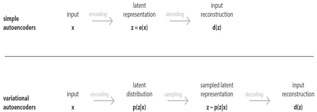
Figure 3.2.3: Difference between a vanilla autoencoder and a Variational Autoencoders (VAE).[66]
