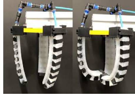
Figure 3.1.6: Hybrid Grippers with soft and rigid structures[53]
