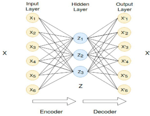
Figure 3.2.1: Architecture of an undercomplete autoencoder.[45]
