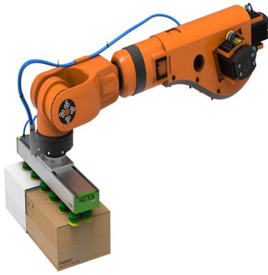
Figure 3.1.1: Vacuum Grippers[55]
