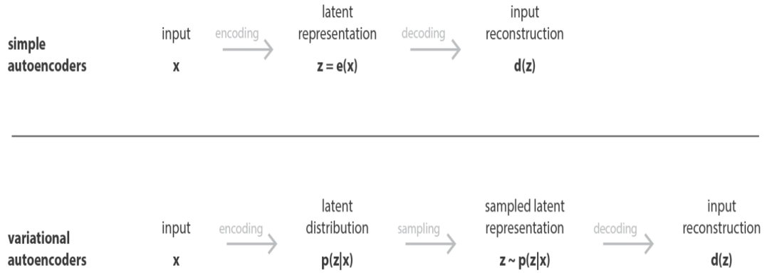
Figure 3.2.3: Difference between a vanilla autoencoder and a Variational Autoencoders (VAE).[65]
