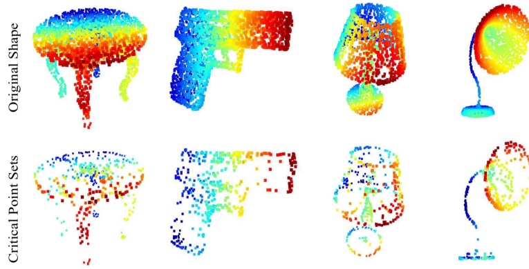
Figure 4.2.2: Critical points set and the original shape.[56]
