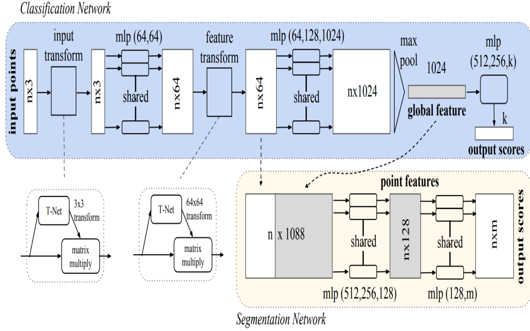
Figure 4.2.1: The PointNet Architecture.[56]
