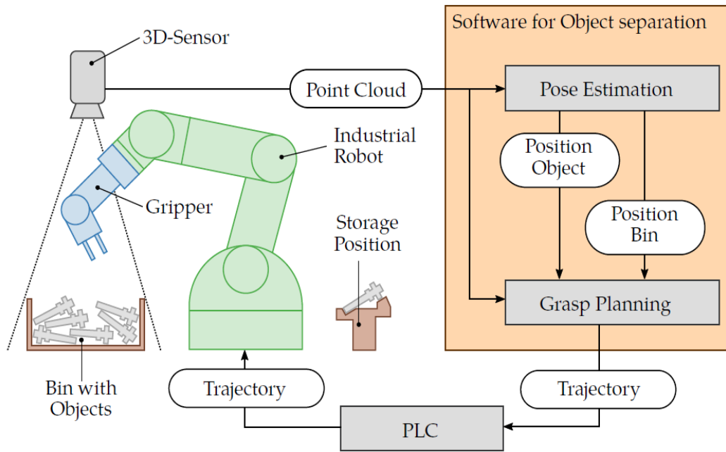
Figure 3.1.7: Overview of model-based bin picking approach.[62]
