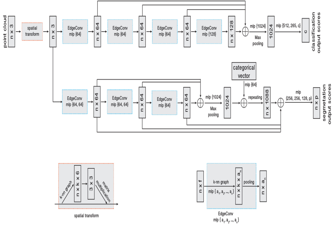
Figure 4.2.3: The DGCNN Architecture.[69]
