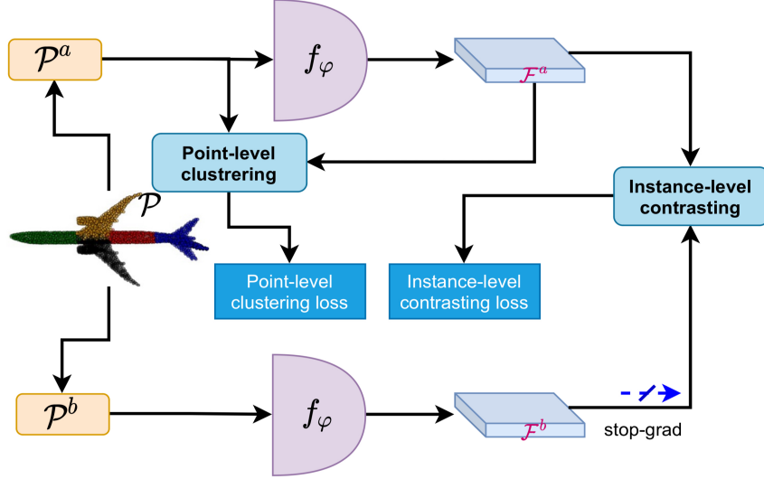
Figure 4.1.1: The Conclu model pipeline including the two modules: point -level clustering and instance-level contrasting.[44]
