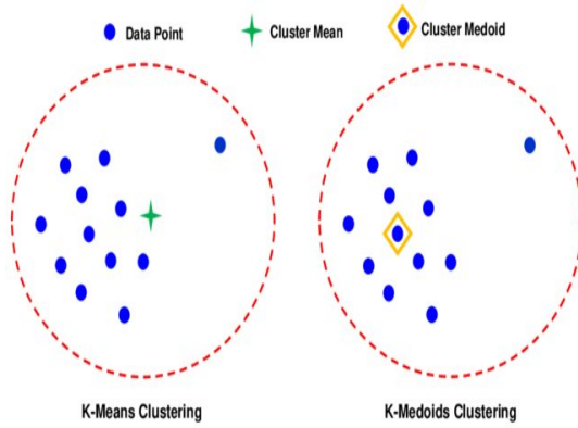
Figure 3.3.2: Difference between K-Means and K-Medoids.[17]
