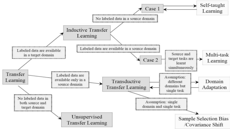
Figure 3.5.3: Overview of the different types of transfer learning.[50]
