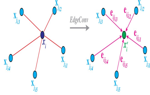
Figure 4.2.5: The EdgeConv operation. The output of EdgeConv is computed by aggregating the features associated with all the edges that originate from each connected vertex. [69]
