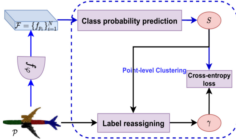
Figure 4.3.1: The architecture of the point-level clustering based unsupervised feature learning.[44]
