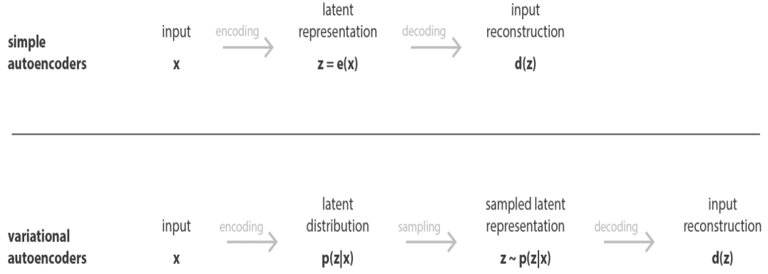
Figure 3.2.4: Difference between a vanilla autoencoder and a Variational Autoencoders (VAE).[85]
