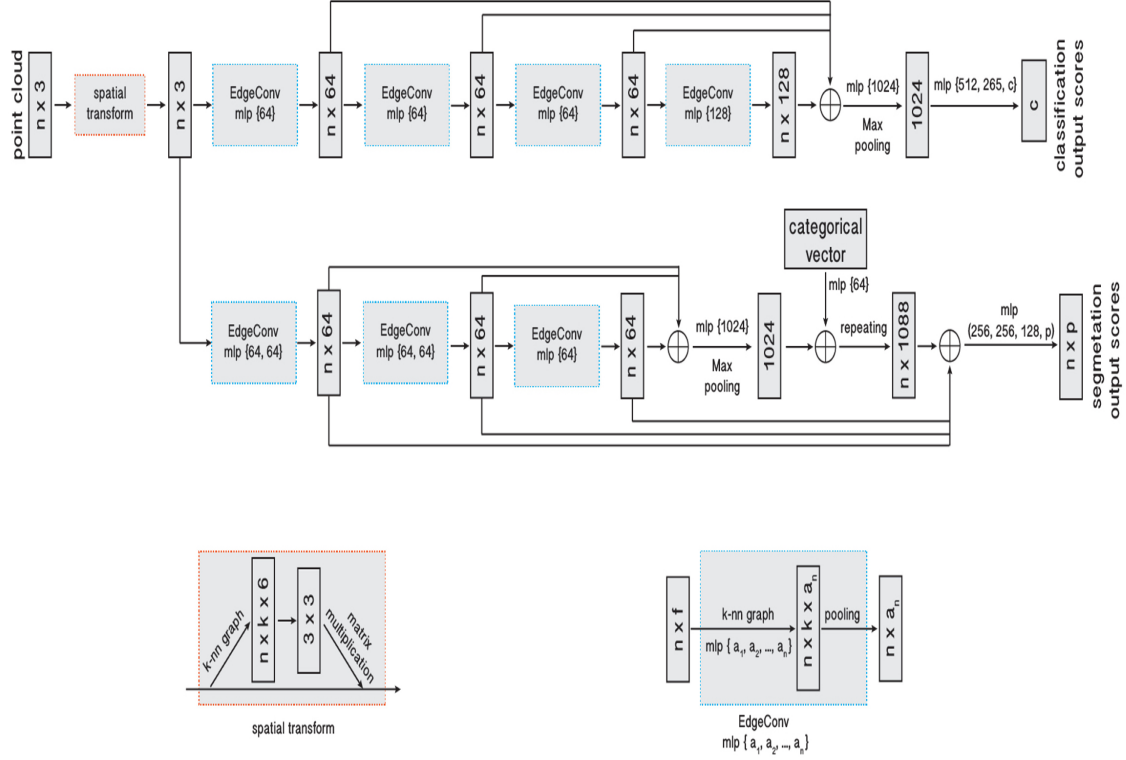
Figure 4.2.3: The DGCNN Architecture.[90]
