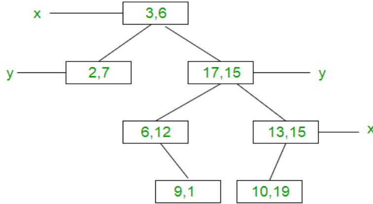
Figure 4.7.1: A demonstration of the KD-tree algorithm with 7 datapoints having 2 dimensions x and y . [69]
