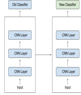
Figure 3.5.2: A model trained on a different task is adapted to be used for a new task.[87]
