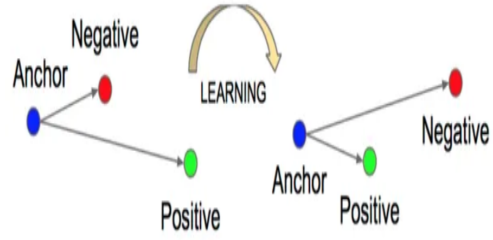
Figure 3.2.5: Before (left) and after (right) minimizing triplet loss function[77]
