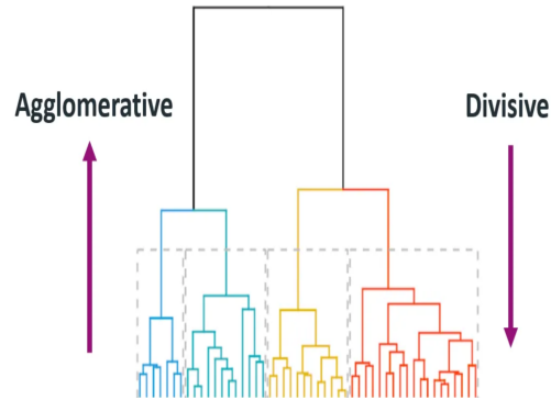
Figure 3.3.3: A dendrogram in hierarchical clustering.[27]
