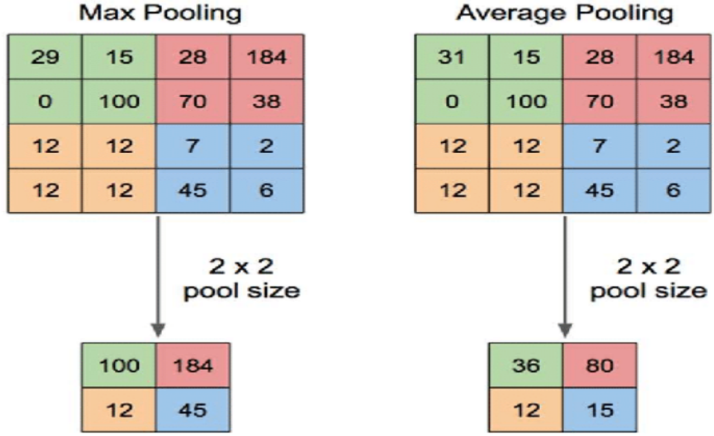
Figure 3.2.1: Max pooling operation on the left and average pooling operation on the right.[94]
