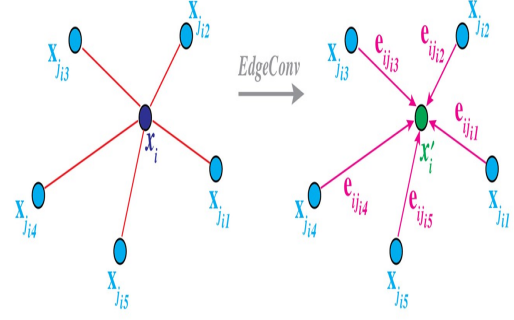
Figure 4.2.5: The EdgeConv operation. The output of EdgeConv is computed by aggregating the features associated with all the edges that originate from each connected vertex. [85]
