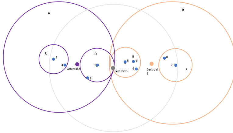
Figure 4.7.2: A demonstration of the Ball-tree algorithm with 9 datapoints having 2 dimensions x and y . [71]
