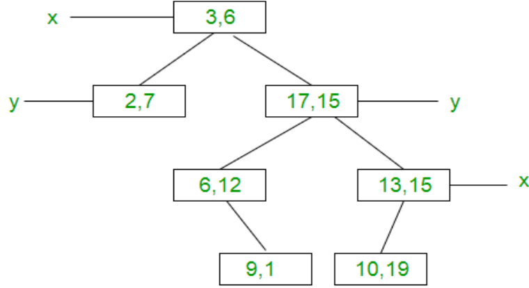
Figure 4.7.1: A demonstration of the KD-tree algorithm with 7 datapoints having 2 dimensions x and y . [71]
