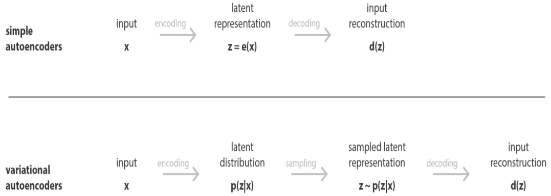
Figure 3.2.4: Difference between a vanilla autoencoder and a Variational Autoencoders (VAE).[80]
