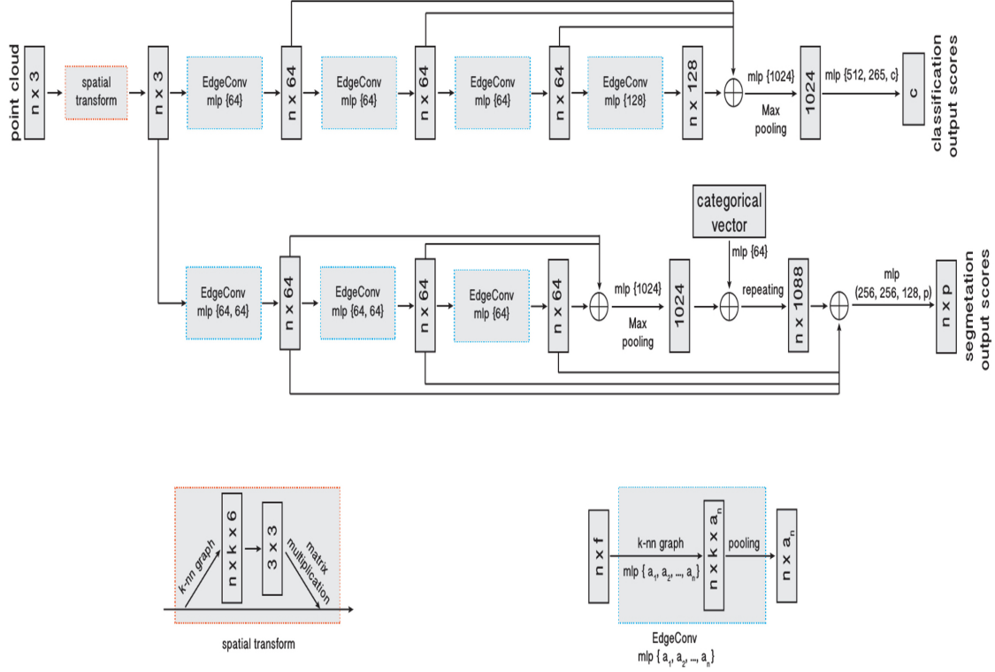
Figure 4.2.3: The DGCNN Architecture.[85]
