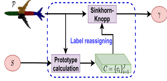
Figure 4.2.3: Architecture of label reassigning [32]
