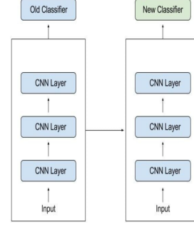
Figure 3.5.2: A model trained on a different task is adapted to be used for a new task.[51]
