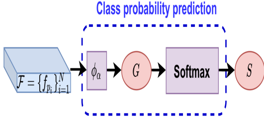
Figure 4.2.2: Architecture of class probability prediction.[32]
