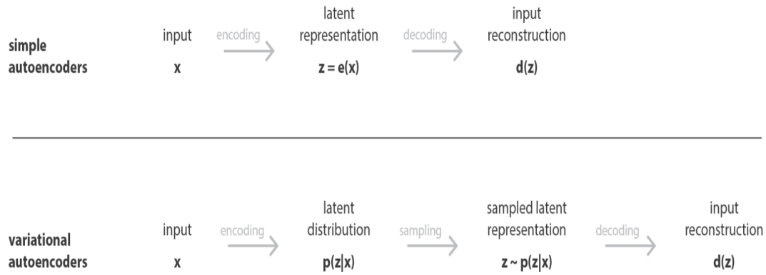
Figure 3.2.3: Difference between a vanilla autoencoder and a Variational Autoencoders (VAE).[45]
