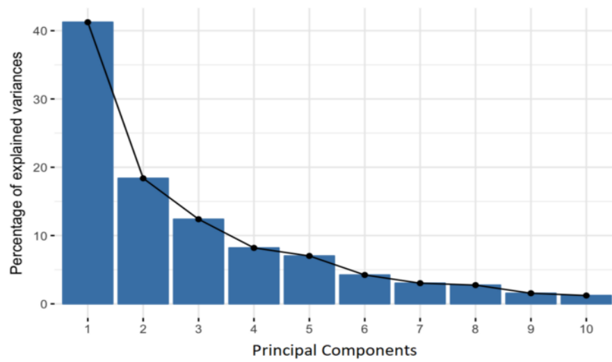
Figure 3.6.4: The percentge of explained variance for each principal component
