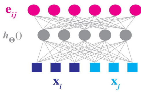
Figure 4.2.4: The Computation of edge feature e_{ij} from a pair of points p_i and p_j . Here, h_\theta is a fully connected layer and the weights associated with it are the trainable parameters \theta . [84]
