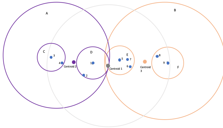
Figure 4.7.2: A demonstration of the Ball-tree algorithm with 9 datapoints having 2 dimensions x and y . [74]
