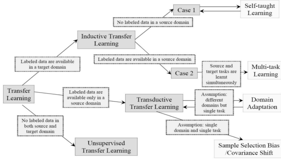
Figure 3.5.3: Overview of the different types of transfer learning.[61]
