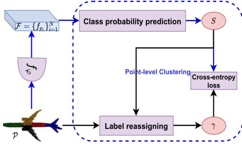
Figure 4.3.1: The architecture of the point-level clustering based unsupervised feature learning.[52]
