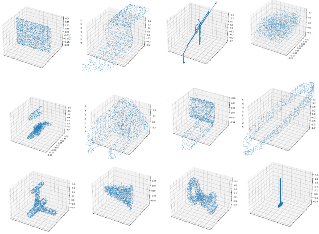
Figure 6.2.1: Some of the representative members of the ABC dataset[41] obtained on applying multi-level HDBSCAN algorithm on the feature representations obtained from the ConClu approach with PointNet Autoencoder backbone.
