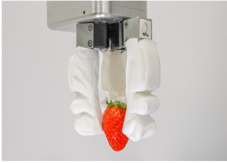
Figure 3.1.5: Soft Grippers[58]
