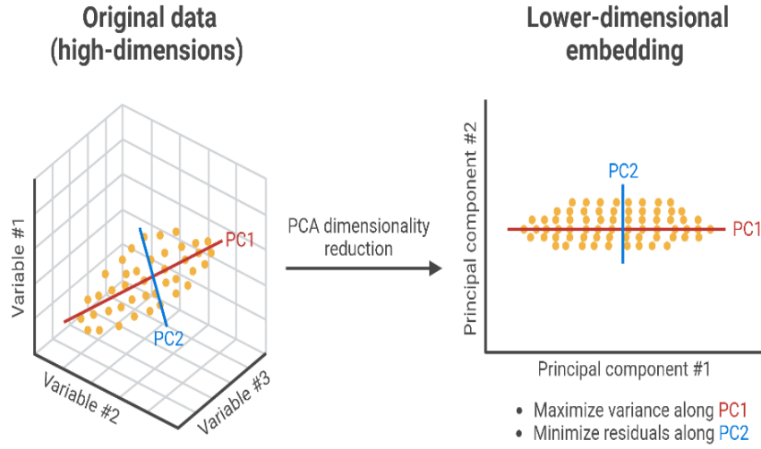
Figure 3.6.3: Projection of the data from higher dimensional space to lower dimensional space on applying PCA[67]
