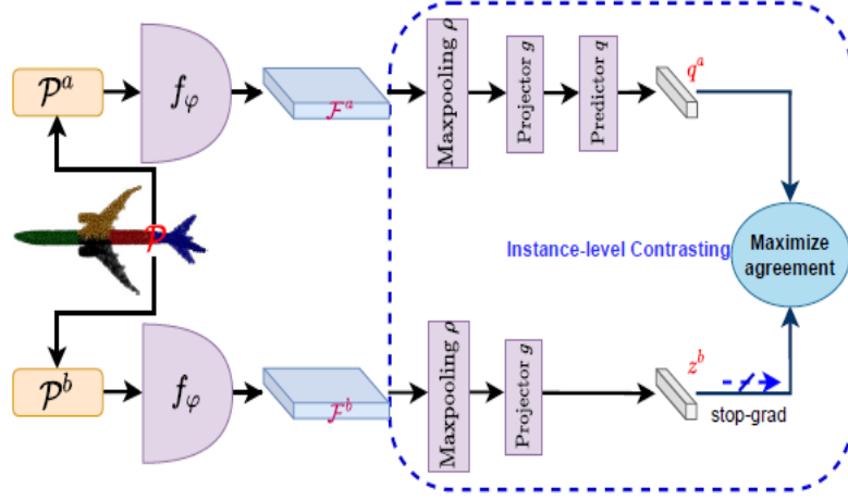
Figure 4.4.1: The architecture of the instance-level Contrasting.[52]
