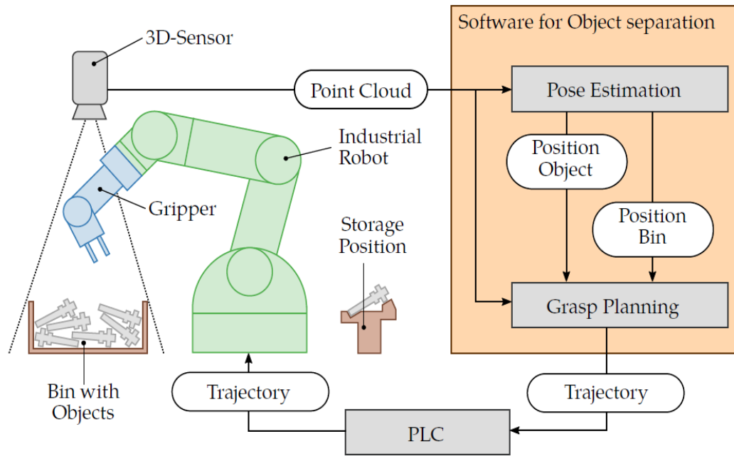
Figure 3.1.7: Overview of model-based bin picking approach.[79]
