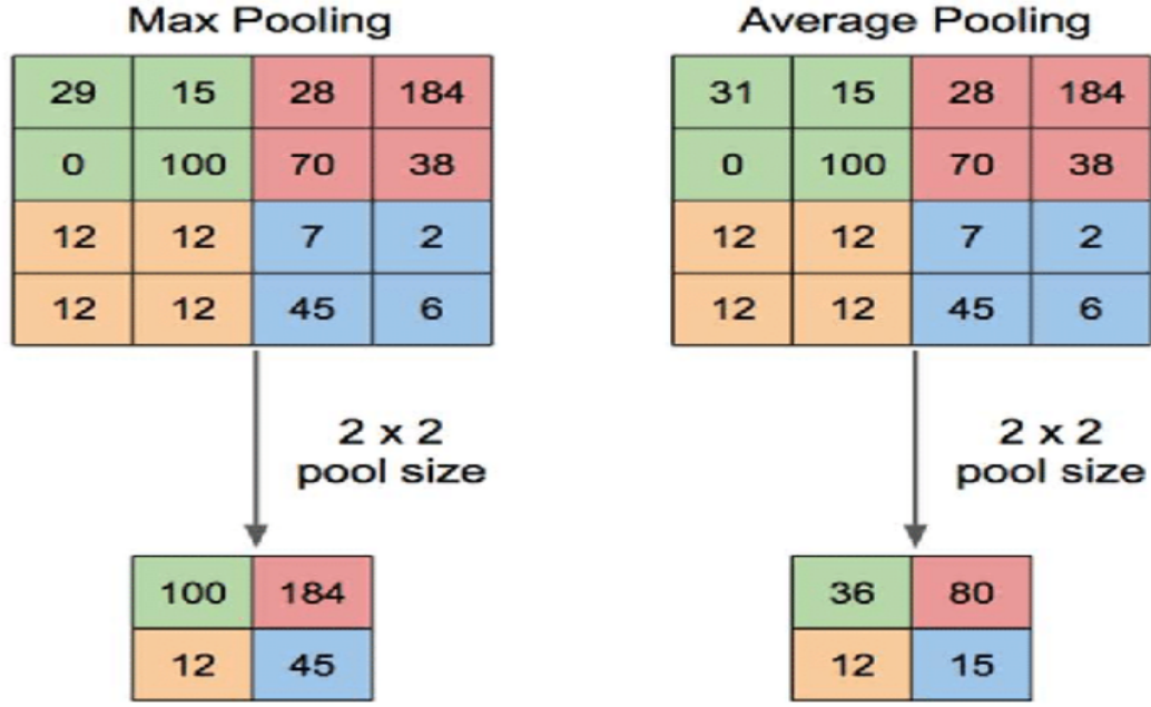
Figure 3.2.1: Max pooling operation on the left and average pooling operation on the right.[97]
