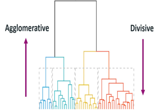
Figure 3.3.3: A dendrogram in hierarchical clustering.[31]
