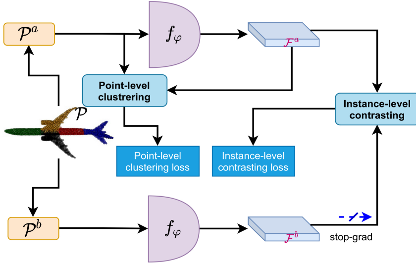
Figure 4.1.1: The Conclu model pipeline including the two modules: point-level clustering and instance-level contrasting.[52]
