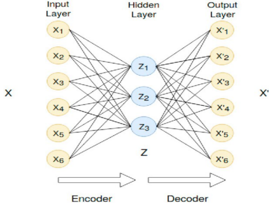
Figure 3.2.2: Architecture of an undercomplete autoencoder.[53]
