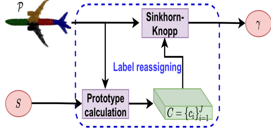
Figure 4.3.3: Architecture of label reassigning [52]
