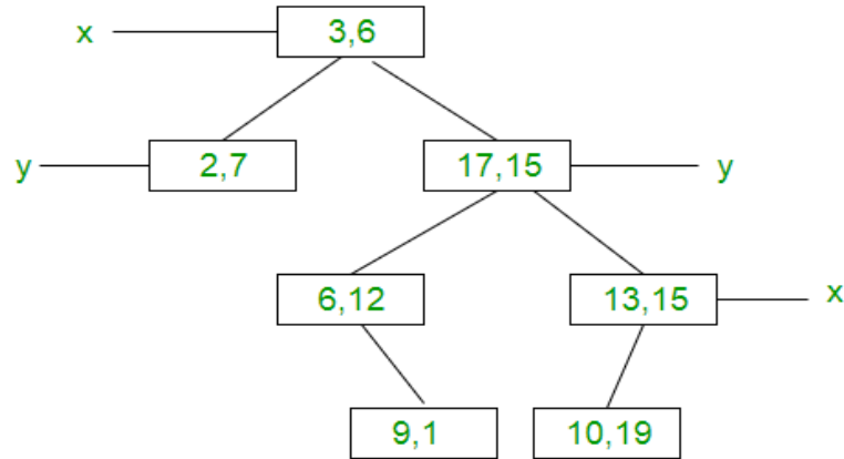
Figure 4.7.1: A demonstration of the KD-tree algorithm with 7 datapoints having 2 dimensions x and y . [74]
