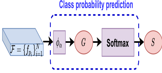
Figure 4.3.2: Architecture of class probability prediction.[35]
