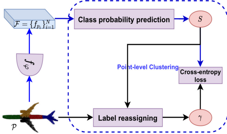
Figure 4.3.1: The architecture of the point-level clustering based unsupervised feature learning.[35]
