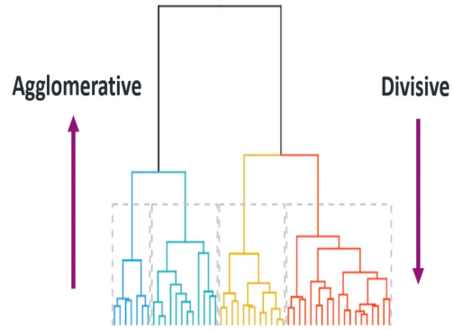
Figure 3.3.3: A dendrogram in hierarchical clustering.[21]
