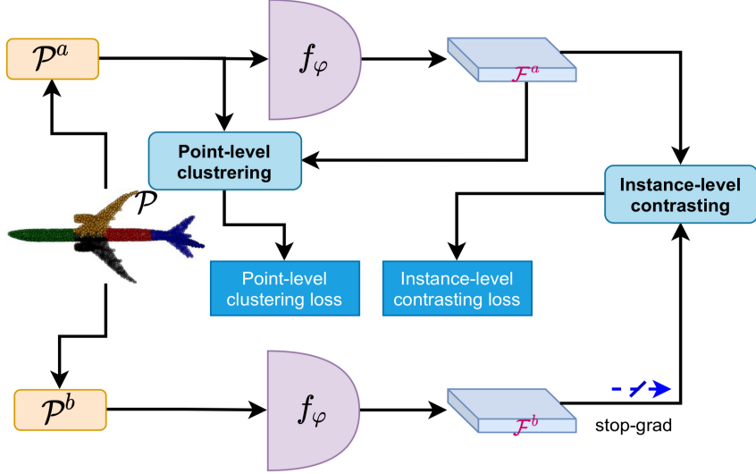
Figure 4.1.1: The Conclu model pipeline including the two modules: point -level clustering and instance-level contrasting.[35]
