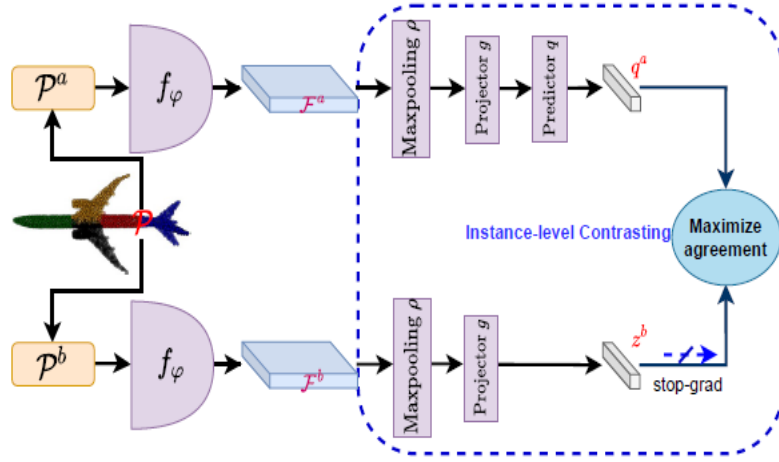
Figure 4.4.1: The architecture of the instance-level Contrasting.[35]
