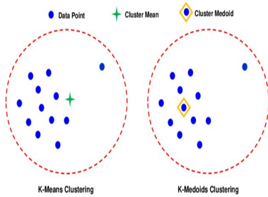
Figure 3.3.2: Difference between K-Means and K-Medoids.[14]
