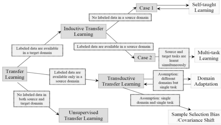
Figure 3.5.3: Overview of the different types of transfer learning.[pan2009survey]
