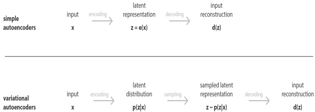
Figure 3.2.3: Difference between a vanilla autoencoder and a Variational Autoencoders (VAE).[vae_image]
