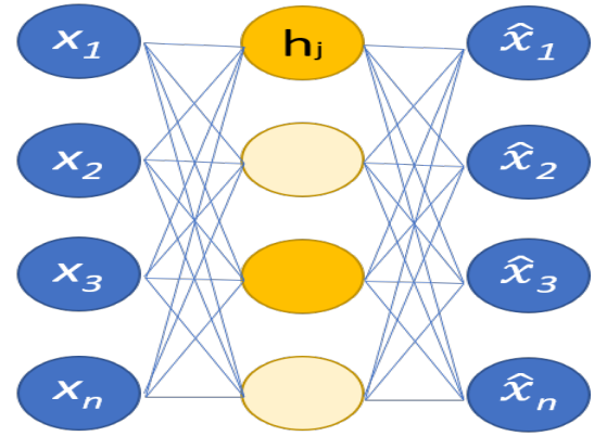
Figure 3.2.2: Architecture of a single layer sparse encoder. The hidden nodes in bright yellow are active, while the ones in light yellow are set to zero, hence inactive[autoencoder]
