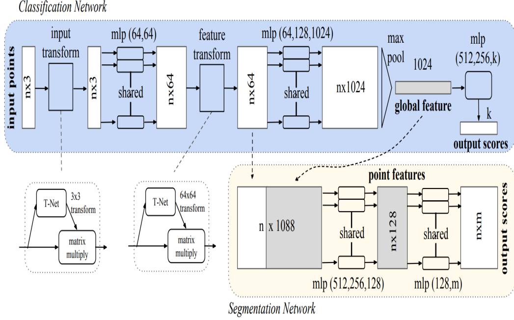
Figure 4.2.1: The PointNet Architecture.[qi2017pointnet]
