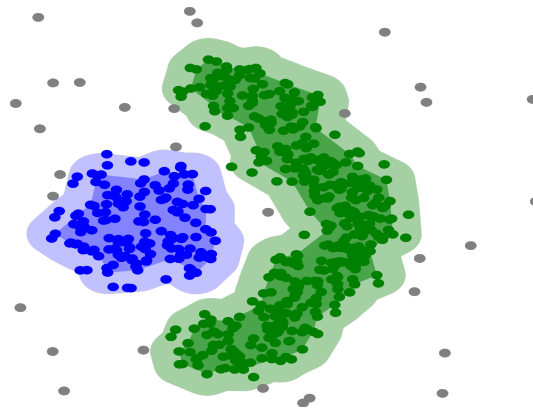
Figure 3.3.1: DBSCAN can find non-linearly separable non-convex clusters.[ dbscanWiki ]
