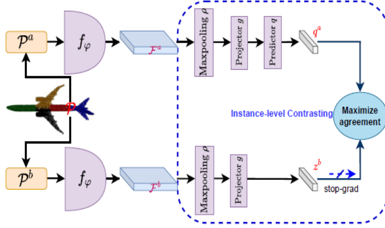
Figure 4.4.1: The architecture of the instance-level Contrasting.[mei2022unsupervised]
