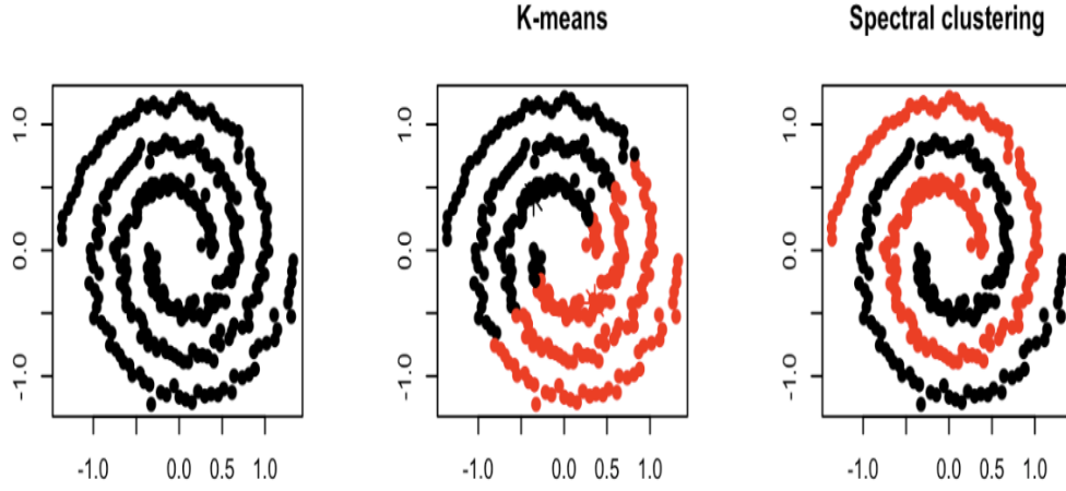
Figure 3.3.4: A comparison between the results of K-means clustering and Spectral clustering. The image in the left shows the points that need to be clustered. [palmer2021spectral]
