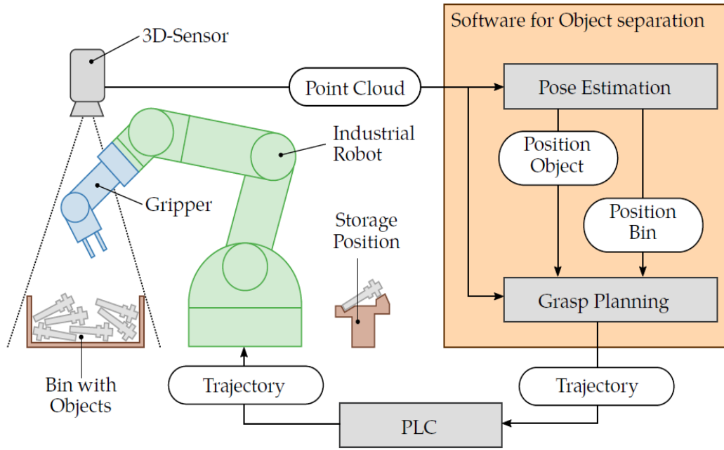
Figure 3.1.7: Overview of model-based bin picking approach.[spenrath2022heuristic]
