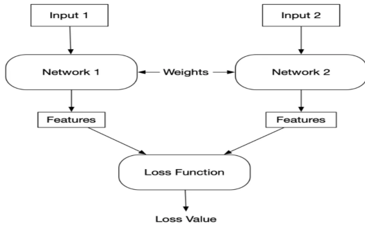
Figure 3.2.4: A generic siamese network.[ siamese_network ]
