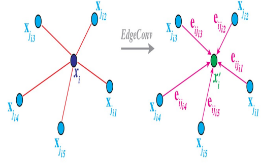
Figure 4.2.5: The EdgeConv operation. The output of EdgeConv is computed by aggregating the features associated with all the edges that originate from each connected vertex. [wang2019dynamic]
