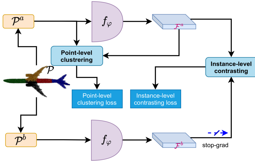
Figure 4.1.1: The Conclu model pipeline including the two modules: point -level clustering and instance-level contrasting.[mei2022unsupervised]
