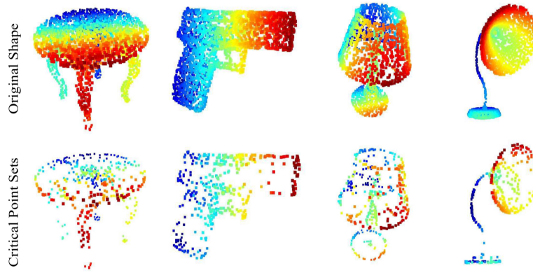
Figure 4.2.2: Critical points set and the original shape.[qi2017pointnet]
