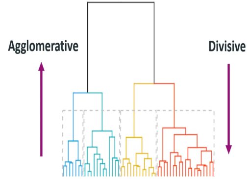
Figure 3.3.3: A dendrogram in hierarchical clustering.[ dendrogram ]
