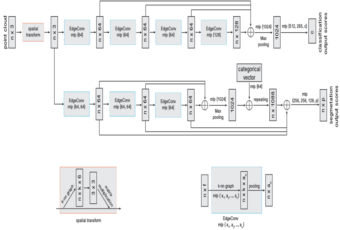
Figure 4.2.3: The DGCNN Architecture.[wang2019dynamic]
