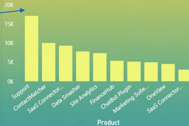
Top 10 Product by Profit
