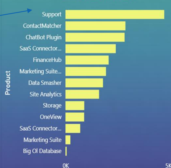
Units Sold by Product
