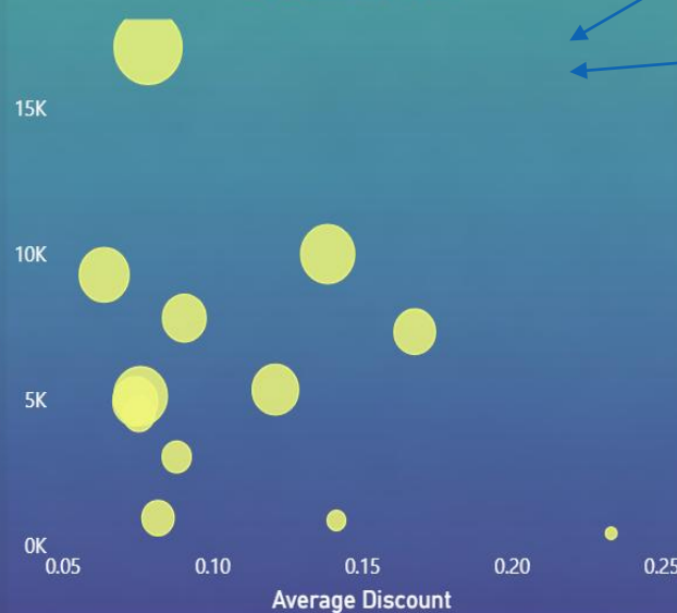
Discount vs Profit
