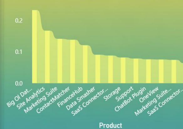
Average Discount Across Products
