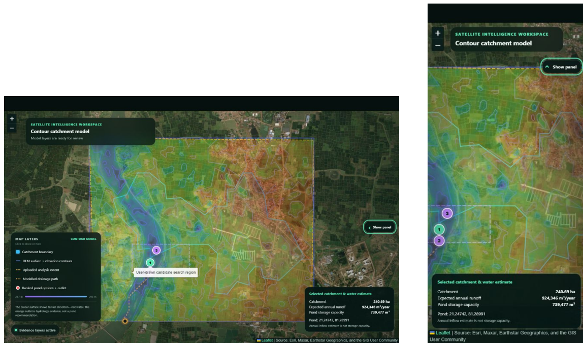
Fig. 4. User-drawn search region after recomputation, shown at desktop and mobile widths. The changed site has 240.69 ha catchment, 924,346 m 3 /year runoff and 739,477 m 3 proposed storage. The dashed search polygon restricts pond placement, not the full upstream catchment.
