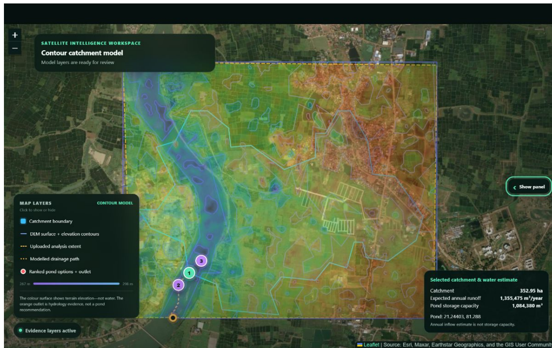
Fig. 3. Fresh allotted-system contour result: coloured DEM, catchment, drainage path and three ranked options, with 352.95 ha catchment, 1,355,475 m 3 /year runoff and 1,084,380 m 3 storage displayed on the map.
